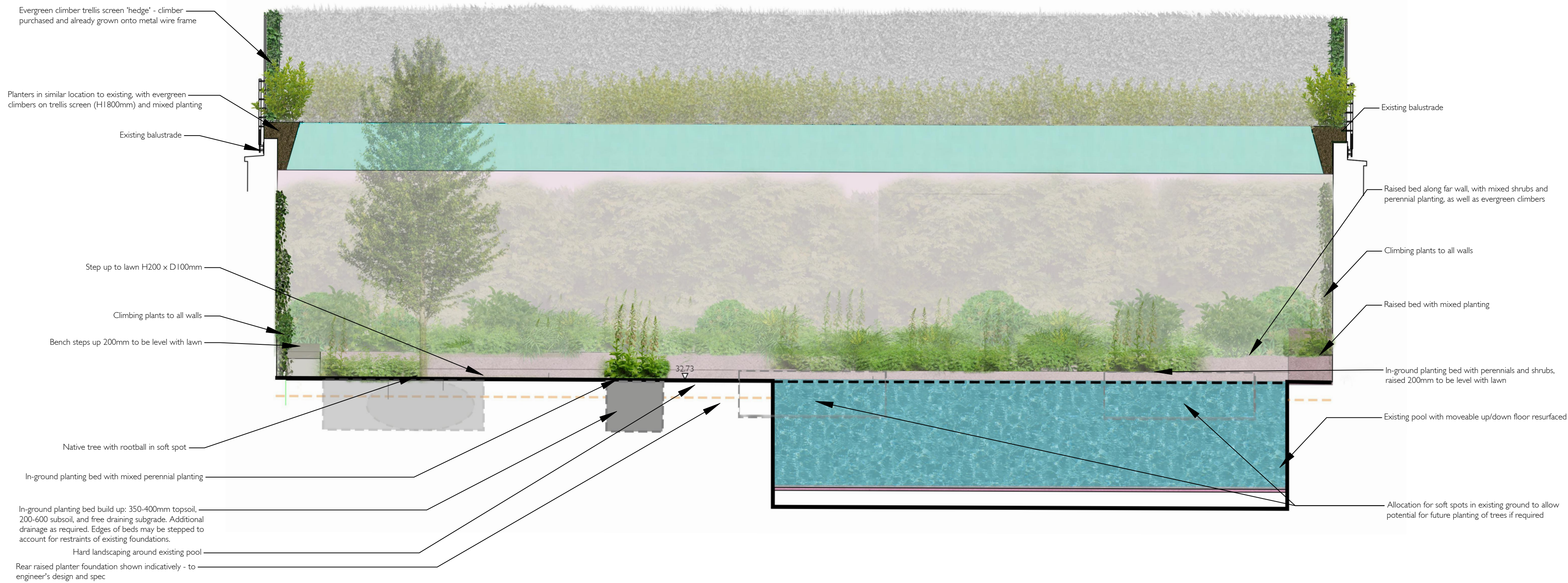
217 01 Landscape sectional elevation E-EE
