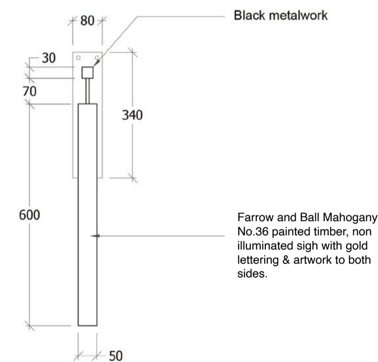
6 Projecting Sign Front Elevation Scale: 1:10
