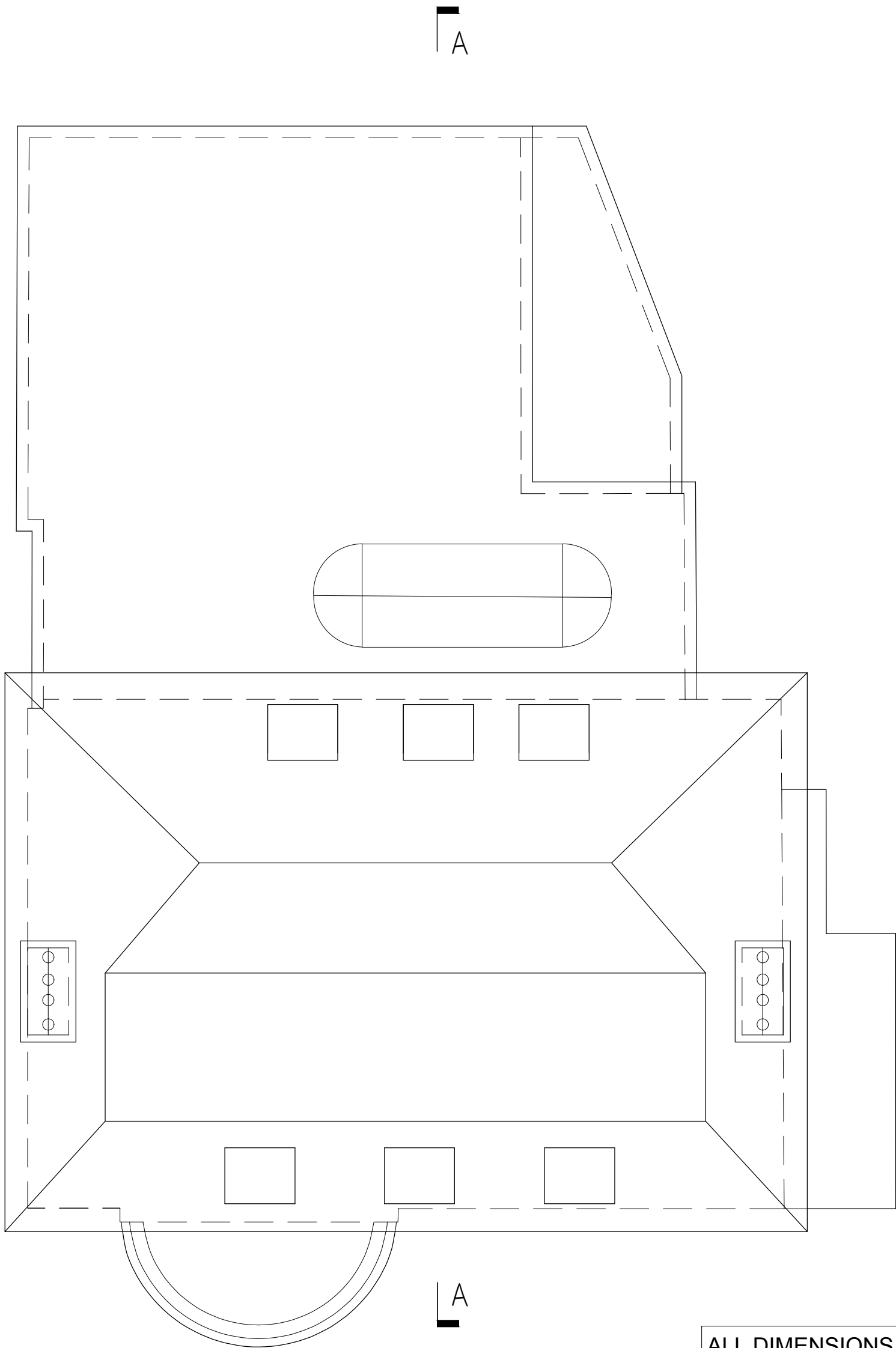
Existing Roof Plan 1:100 @ A3
