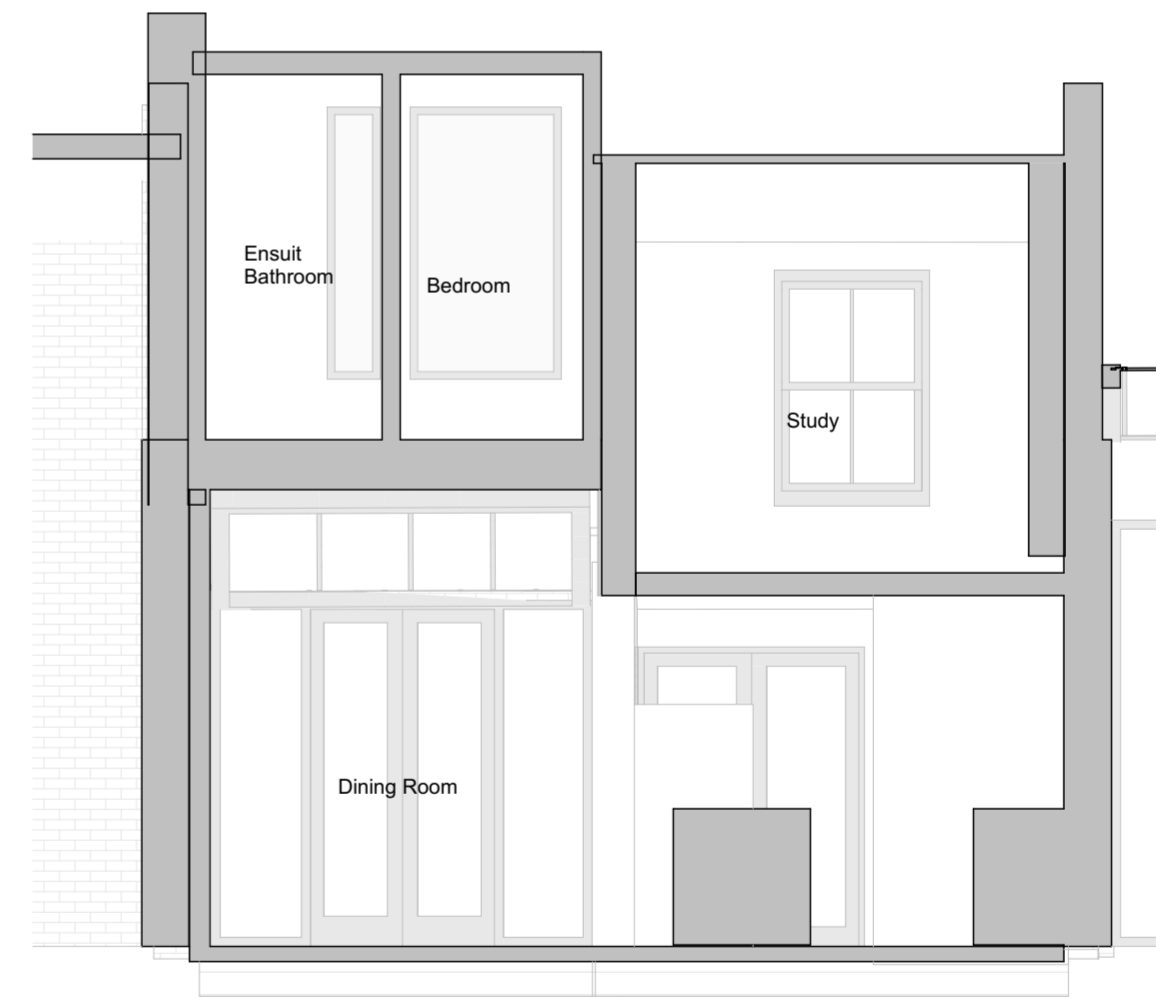
05 Proposed Section B 1:50
