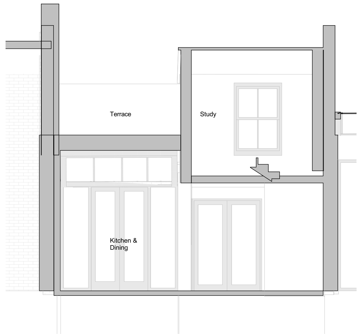
05 Existing Section B
