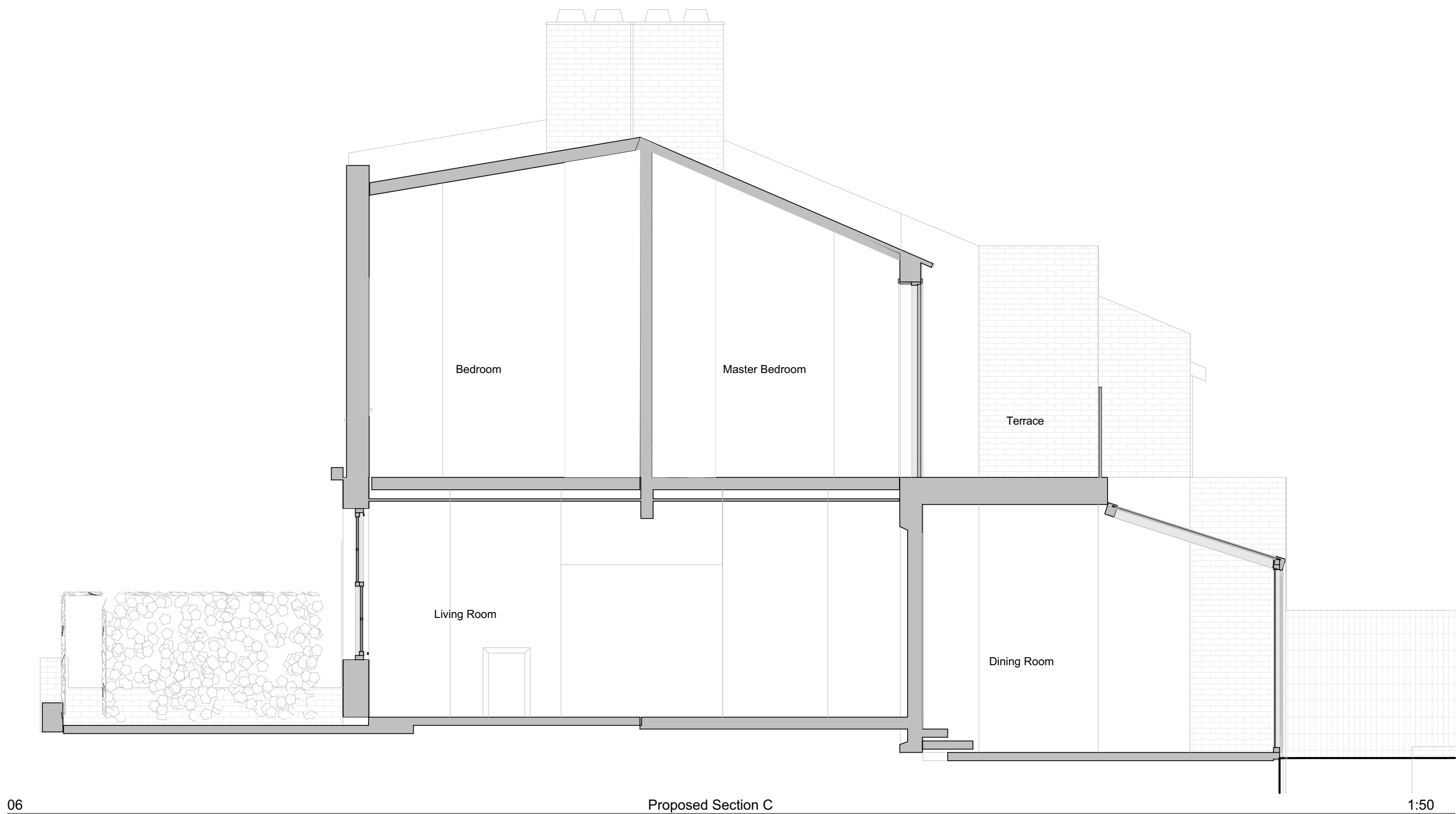
06 Proposed Section C
