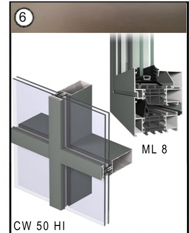
6 RESIDENTIAL DOUBLE GLAZED ALUMINIUM WINDOWS & DOORS: Reynaers CW 50 HI (ground floor) & Reynaers ML 8 (all upper floors).
