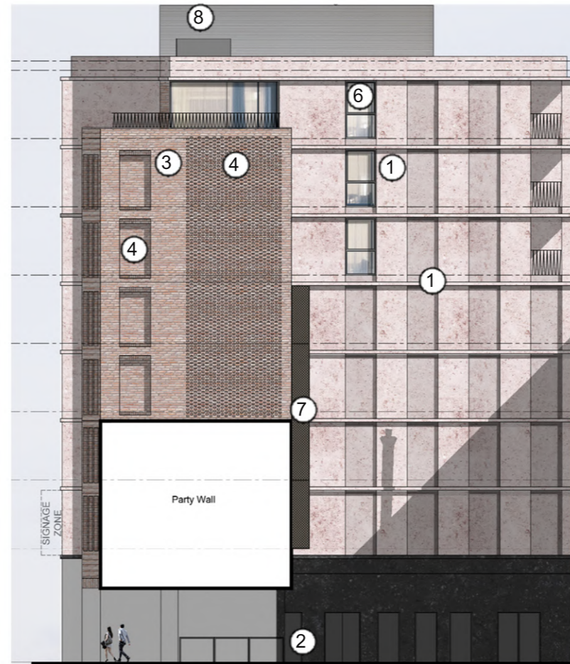
North Elevation
