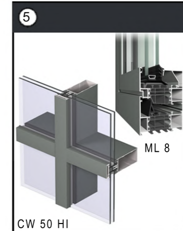
5 HOTEL DOUBLE GLAZED ALUMINIUM WINDOWS & DOORS: Reynaers CW 50 HI (ground floor) & Reynaers ML 8 (all upper floors). RAL 7021 matt
