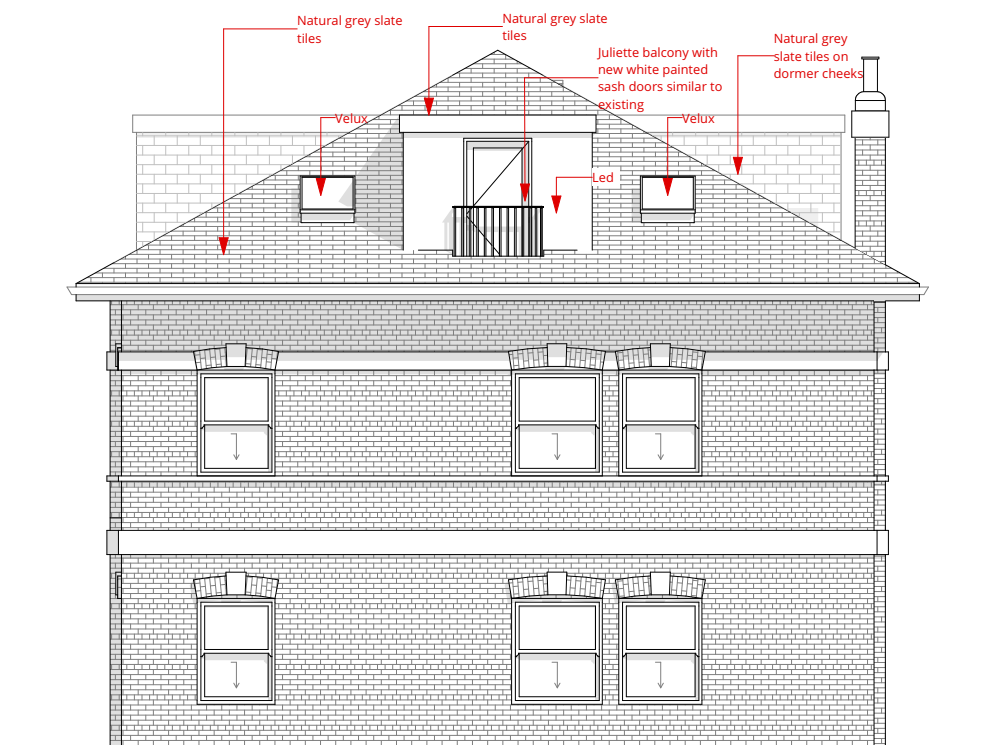
Proposed South Elevation (Back)
