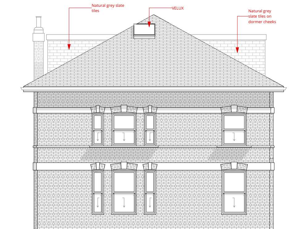
Proposed North Elevation (Front)
