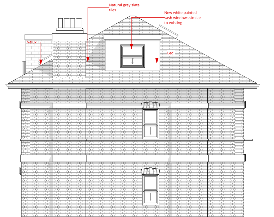
Proposed East Elevation (Side)
