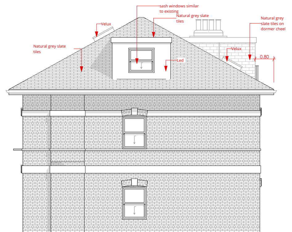
Proposed West Elevation (Side)
