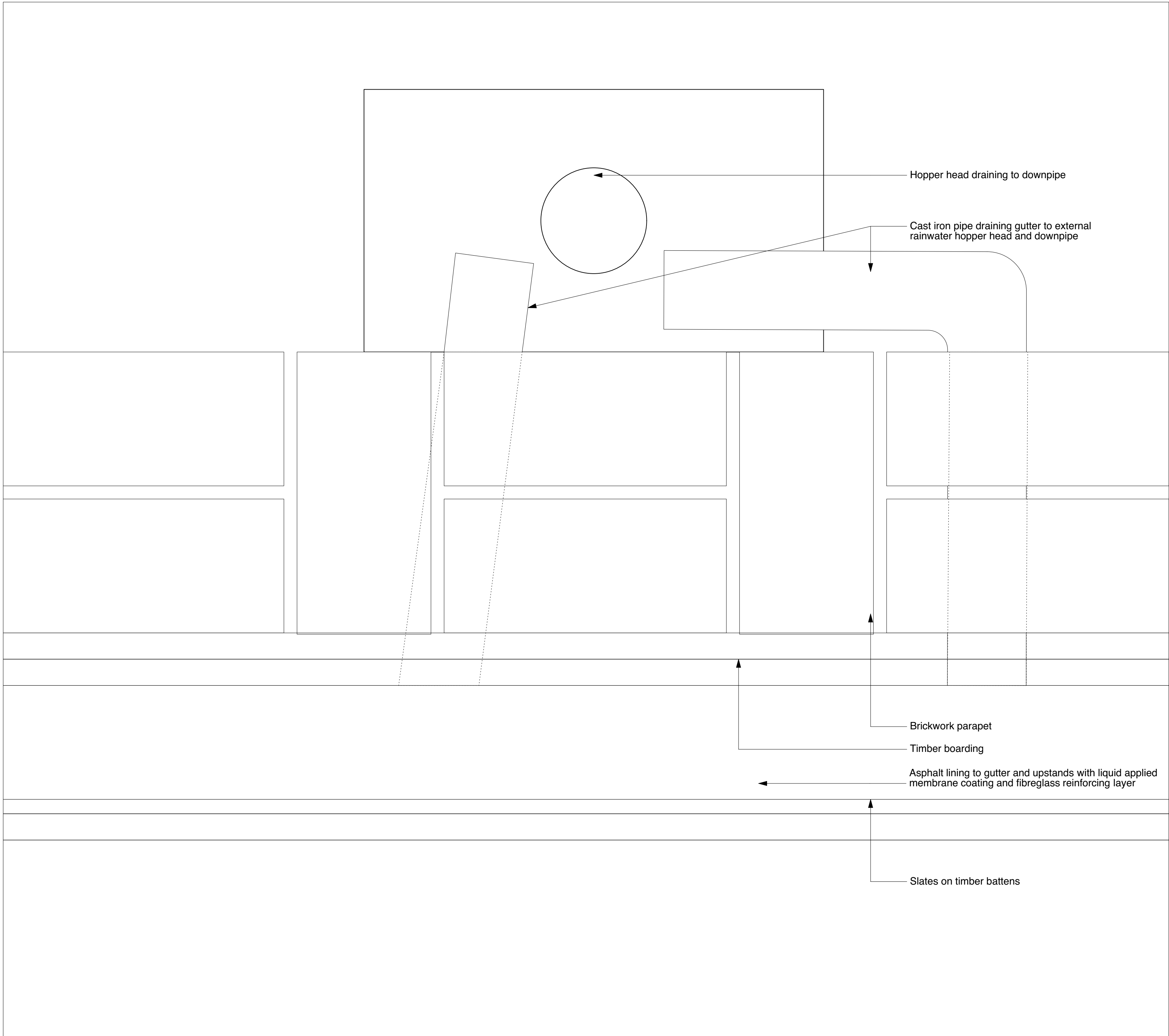
Pre-Existing Plan Detail Scale: Half Actual Size
