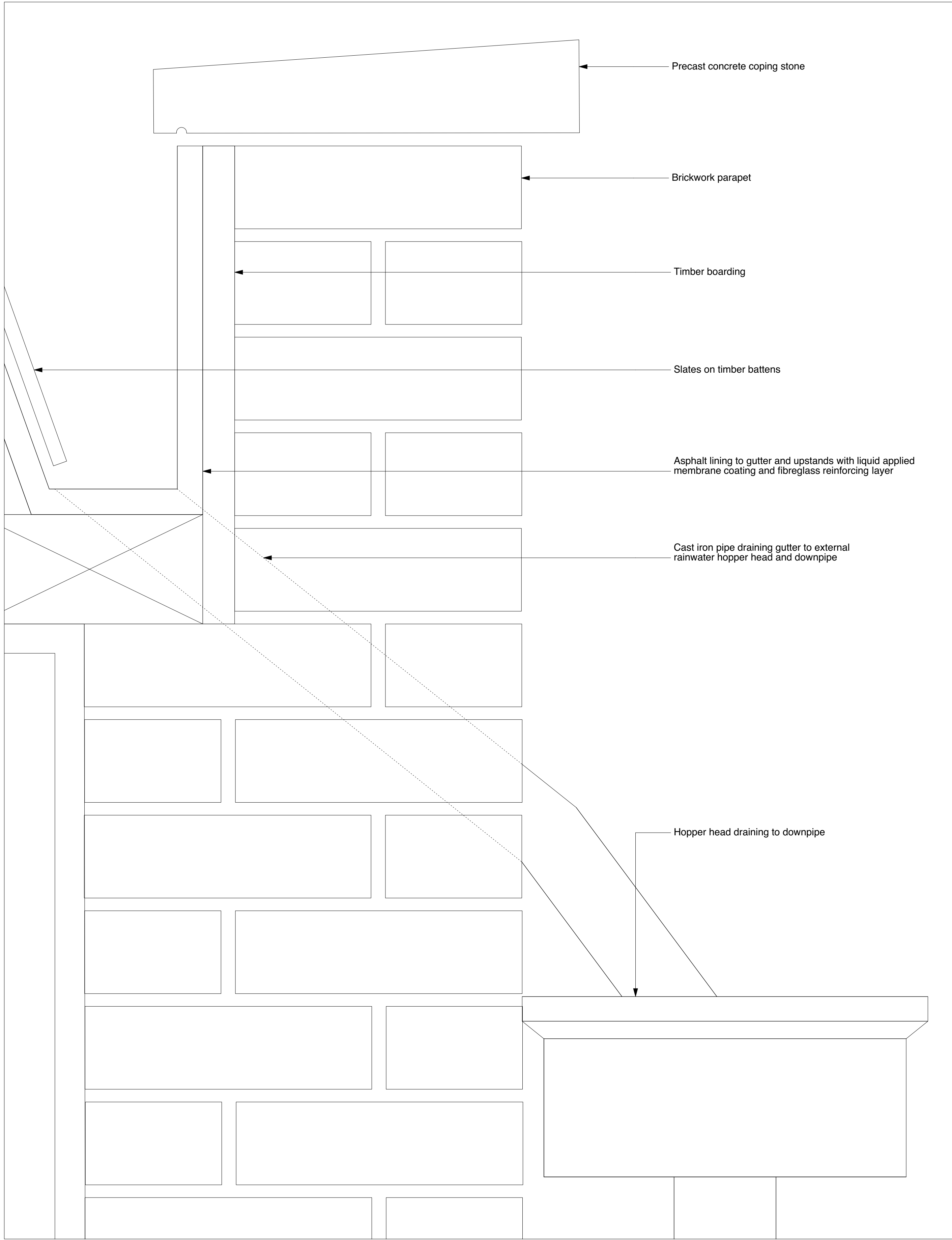
Pre-Existing Section Detail Scale: Half Actual Size
