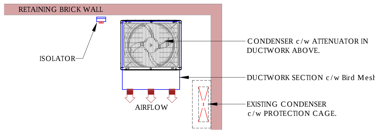
PART PLAN
