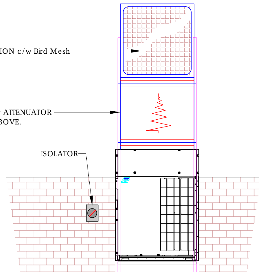
FRONT ELEVATION
