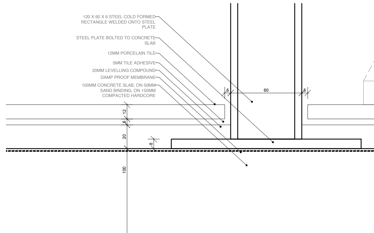
DETAIL 9 Steel column to slab
