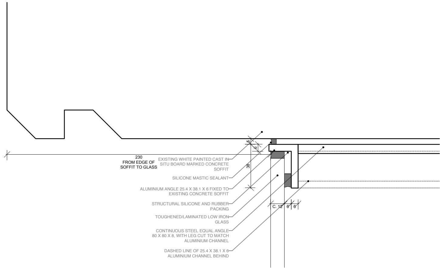
DETAIL 5 Aluminium profile to existing soffit (section)
