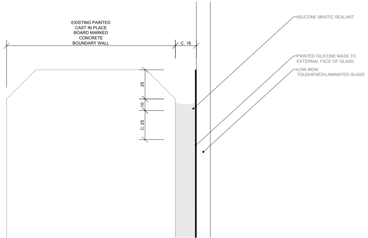
DETAIL 3.2 Glass to top of existing boundary wall (section)
