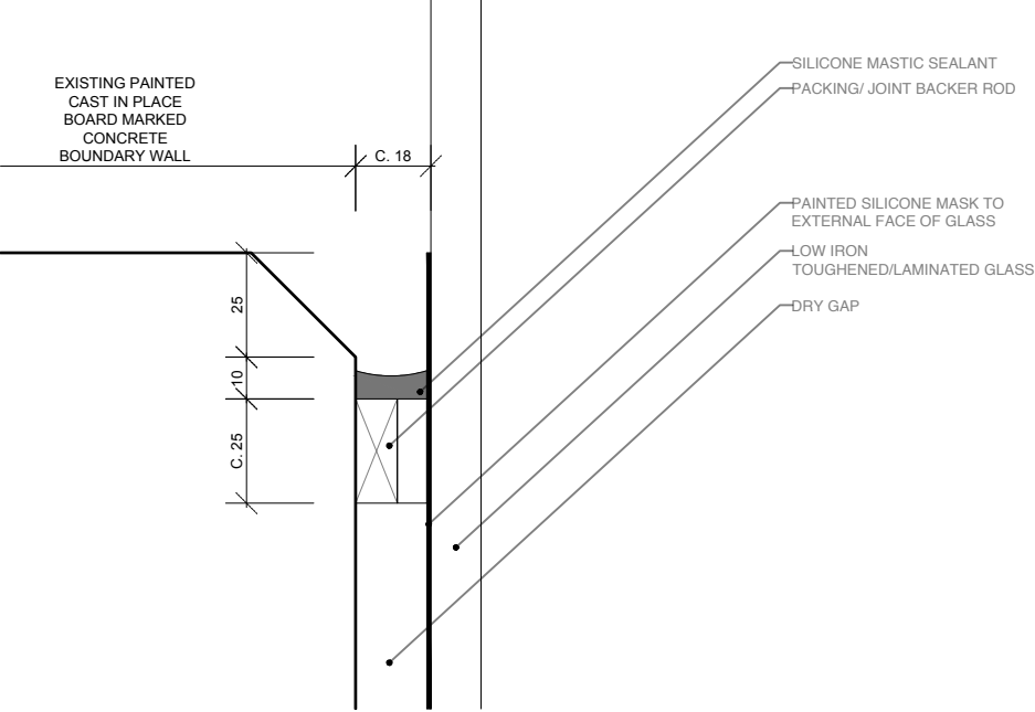
DETAIL 3 Glass to top of existing boundary wall (section)
