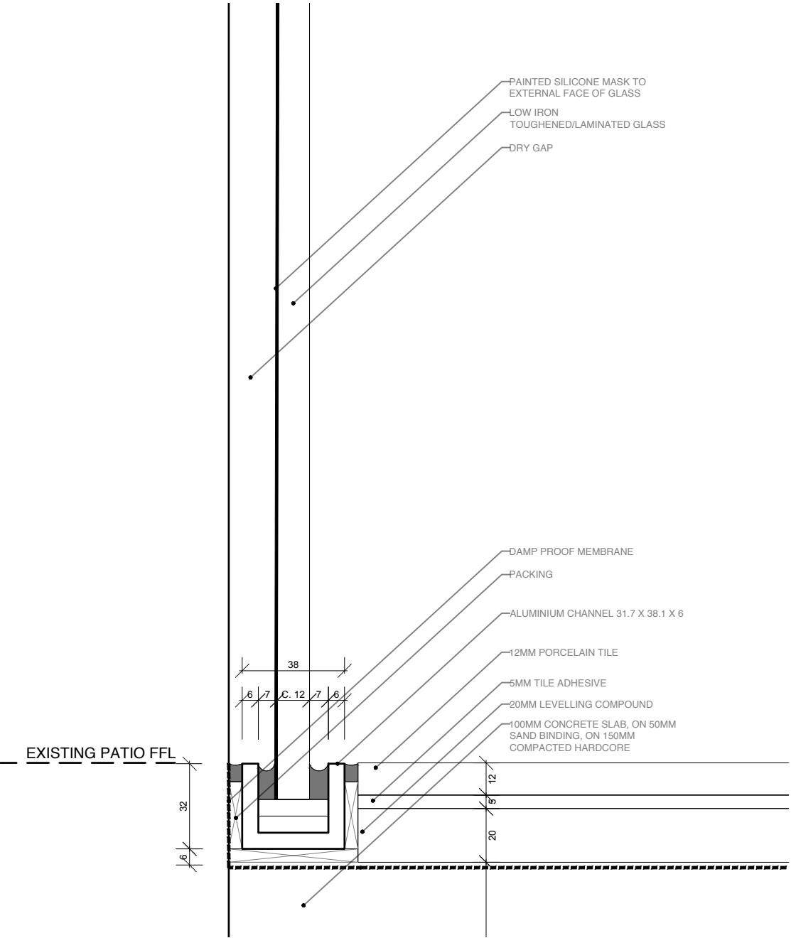
DETAIL 2 Perimeter detail to existing boundary wall (section)
