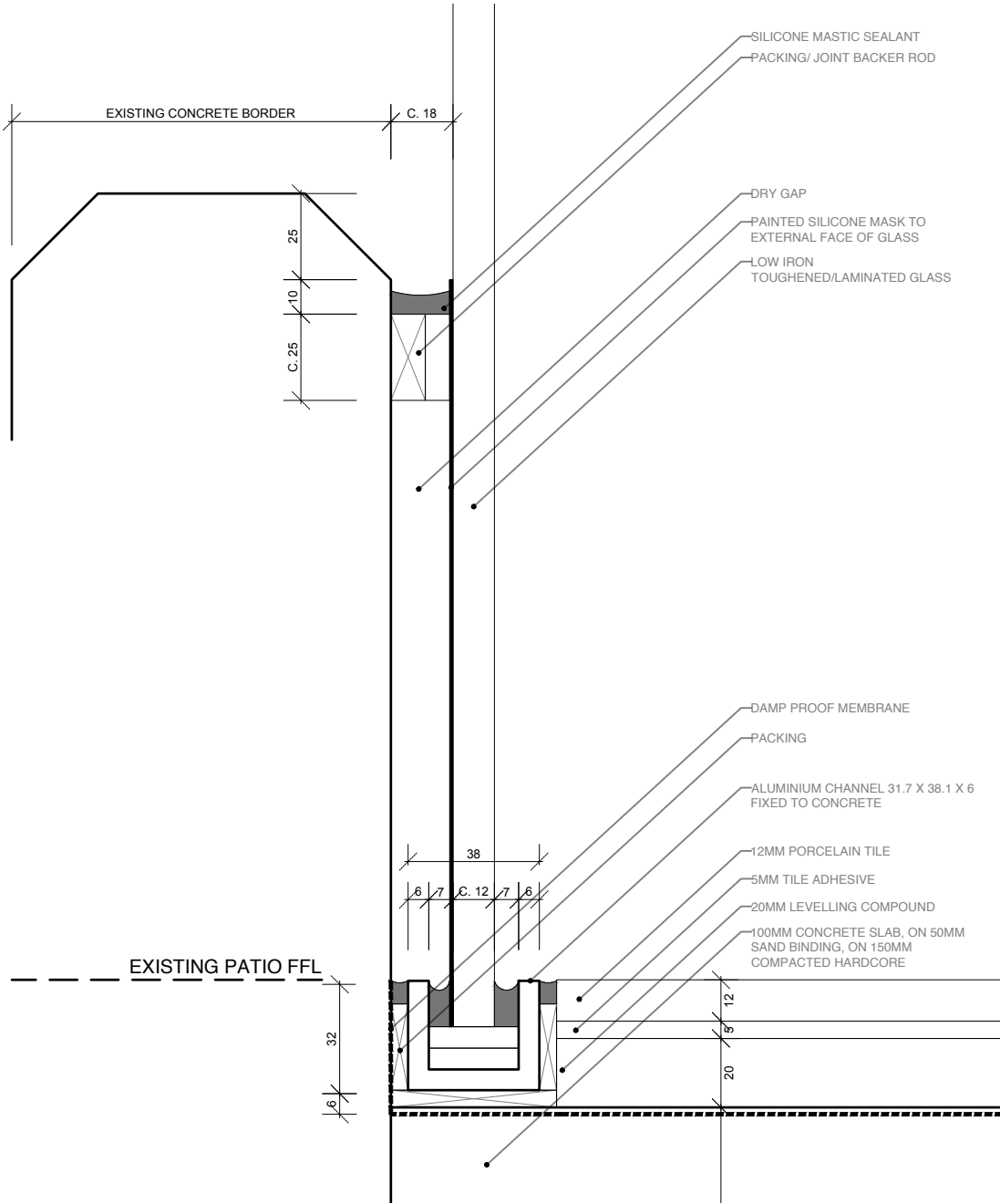
DETAIL 1 Perimeter detail to existing low border wall (section)
