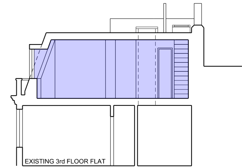
PROPOSED SECTION 'C C'
