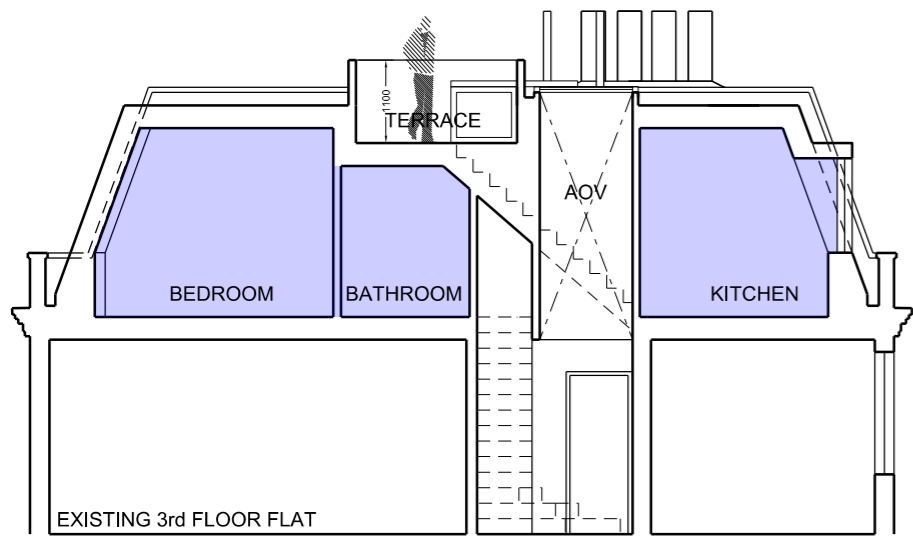
PROPOSED SECTION 'B B'
