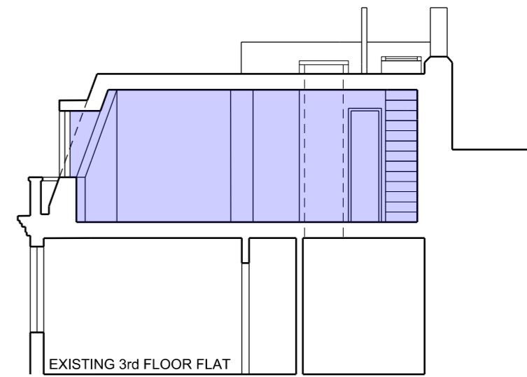
PROPOSED SECTION 'C C'
