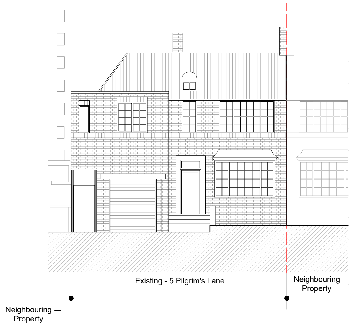
Front Elevation
