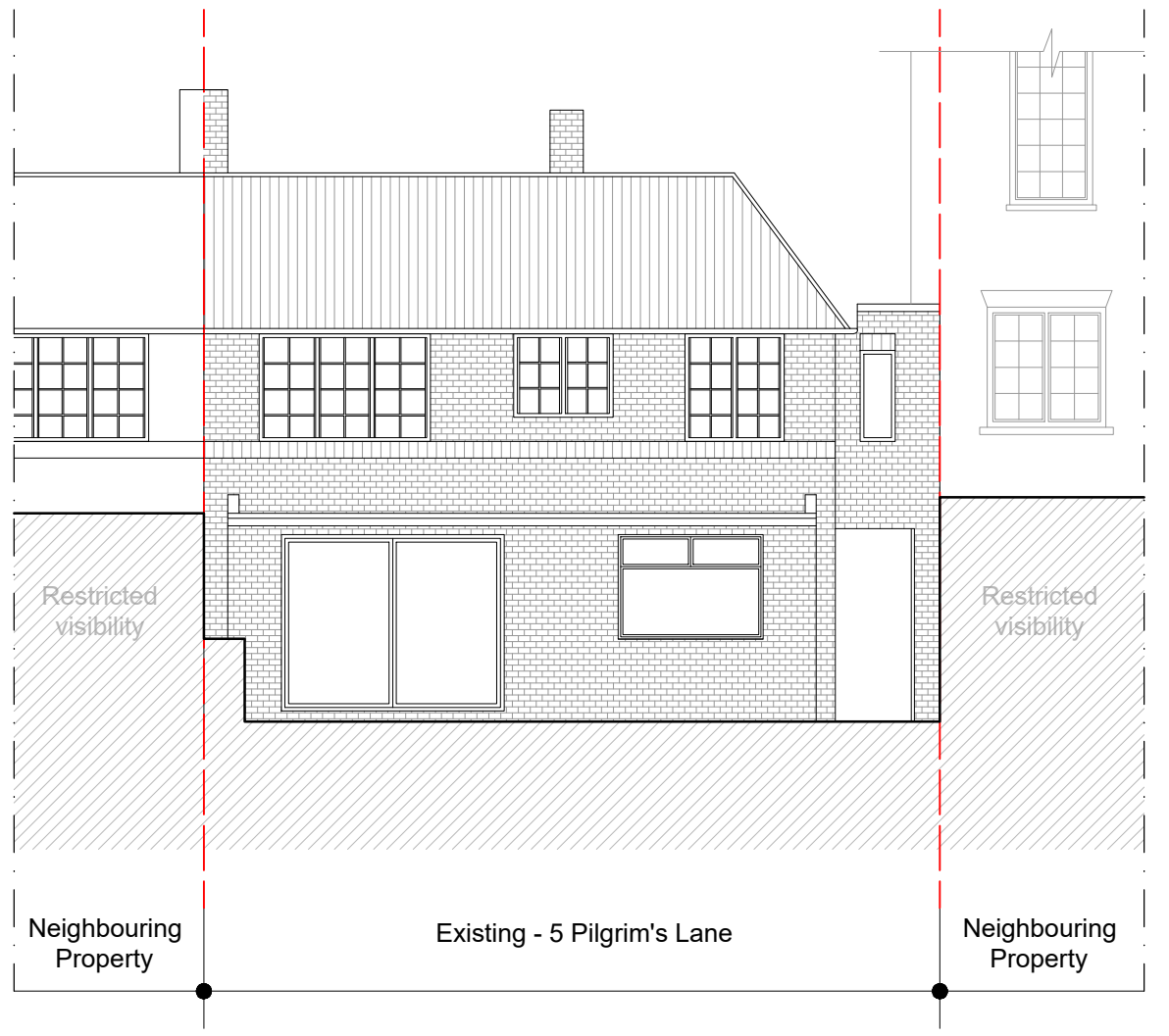
Rear Elevation
