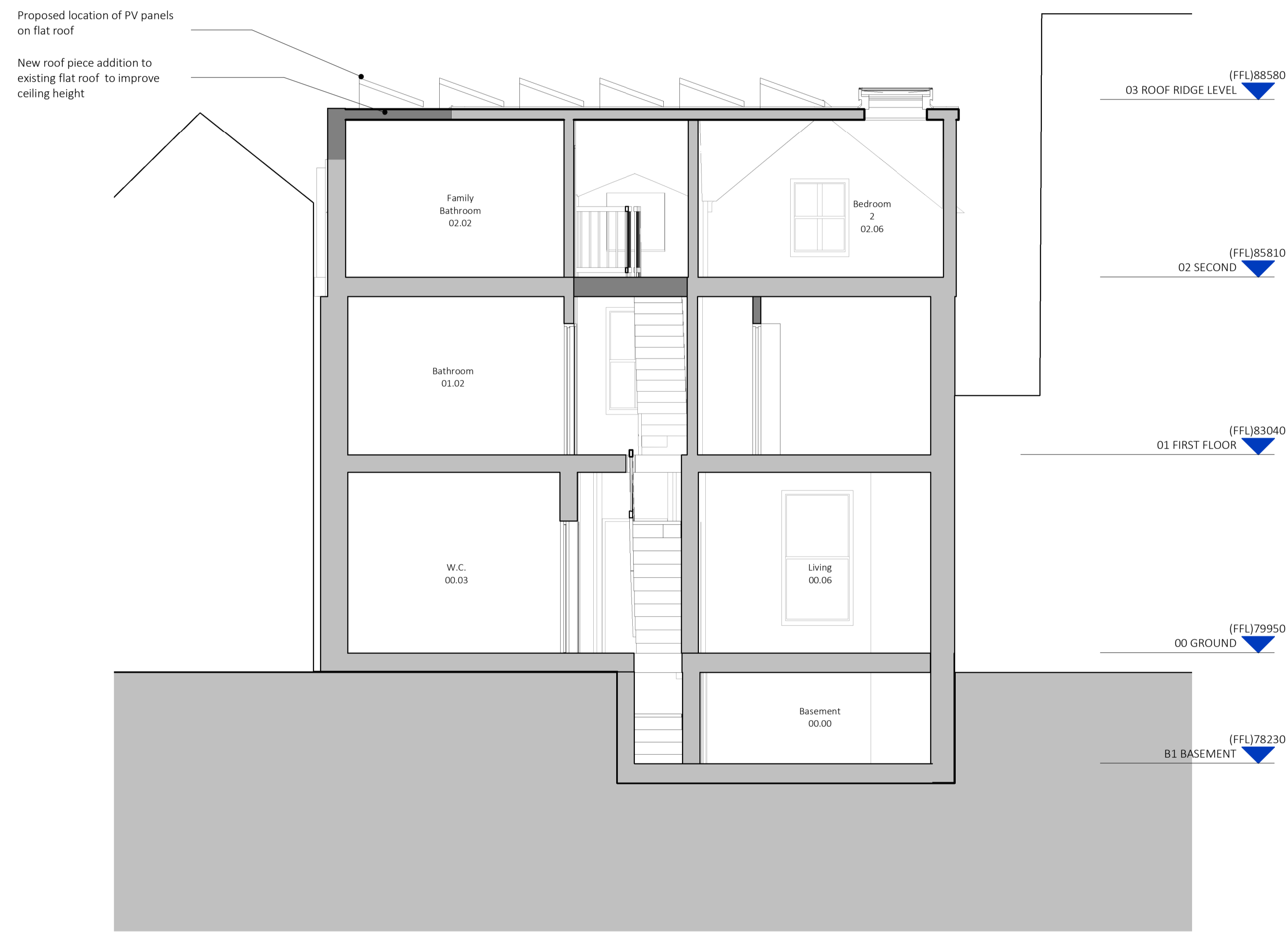
1 1 : 50 PROPOSED SECTION B-B
