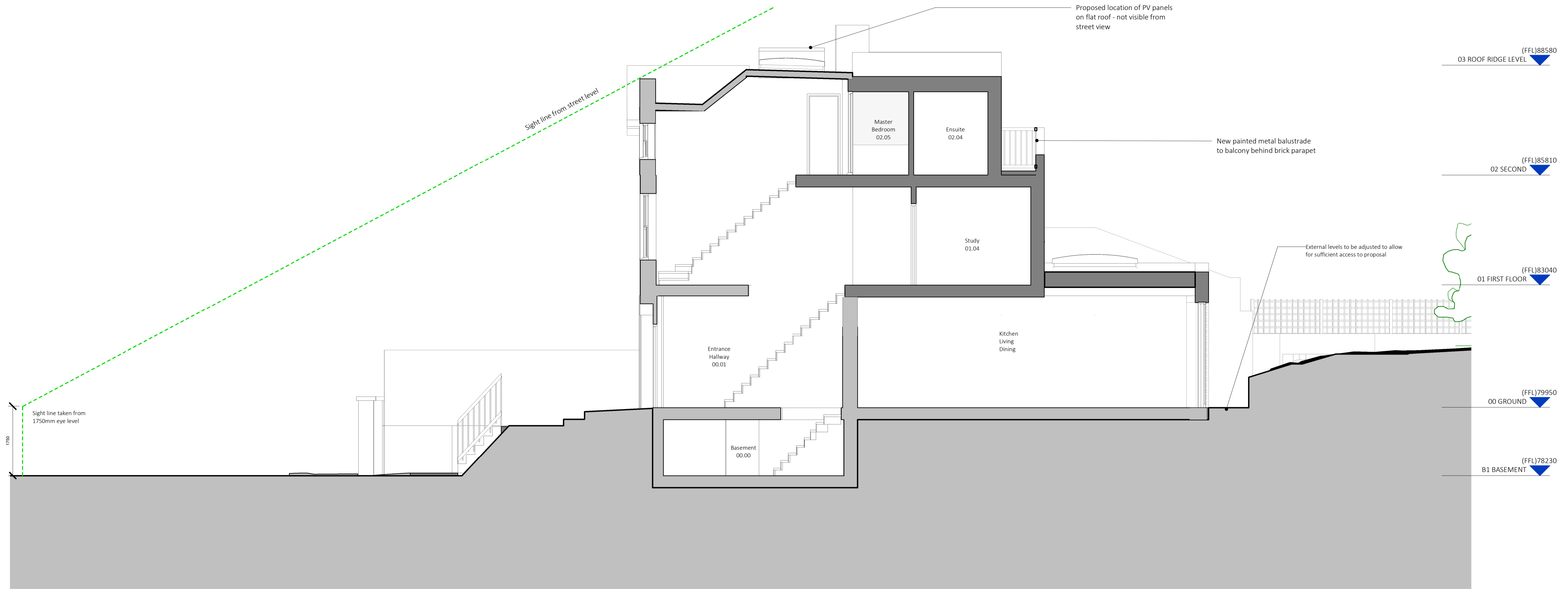
1 1 : 50 PROPOSED SECTION A-A
