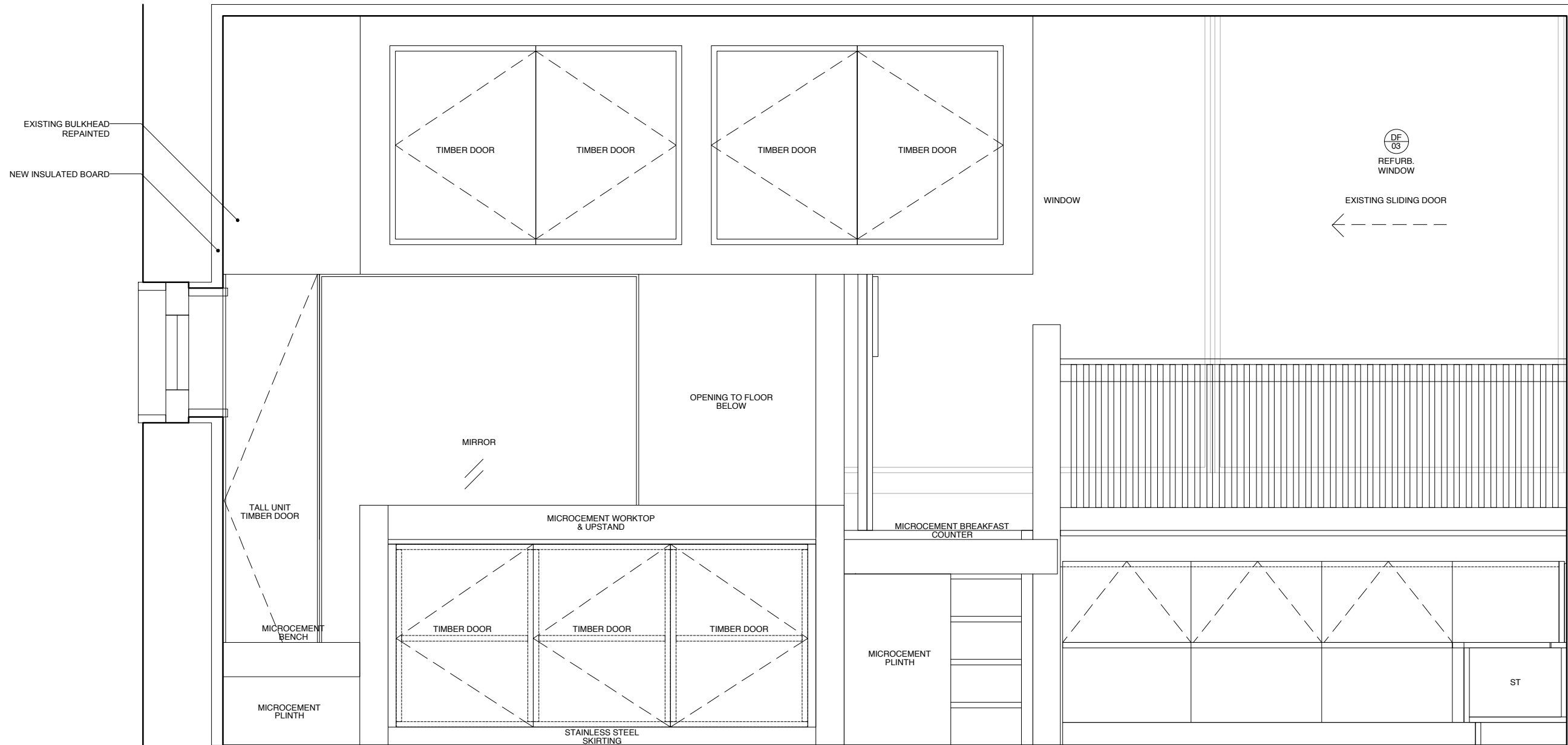
KITCHEN ELEVATION A
