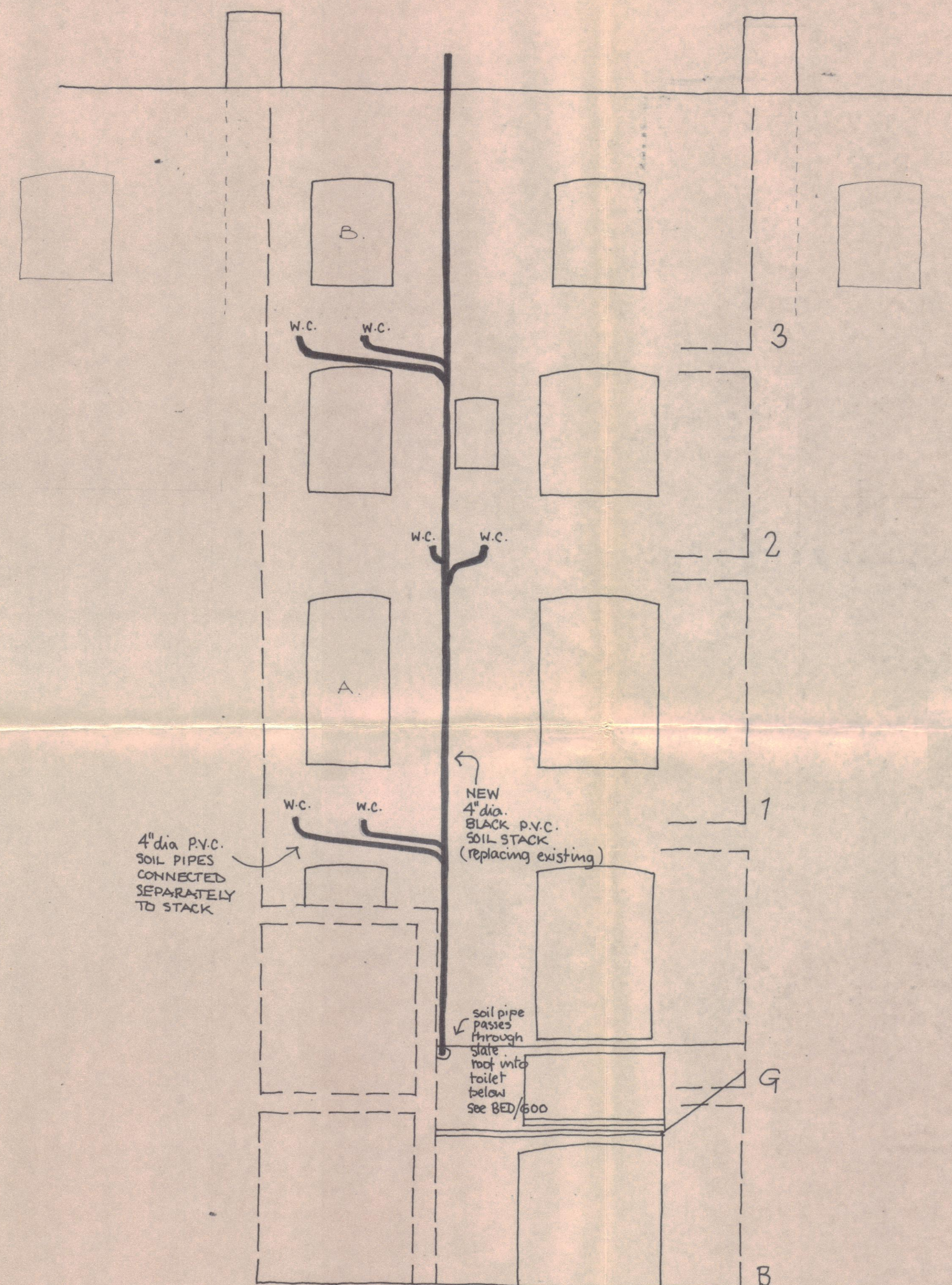
REAR ELEVATION 1/4" to 1'-0" scale. SHOWING SOIL STACK - ALL OTHER PLUMBING RUN INTERNALLY.
