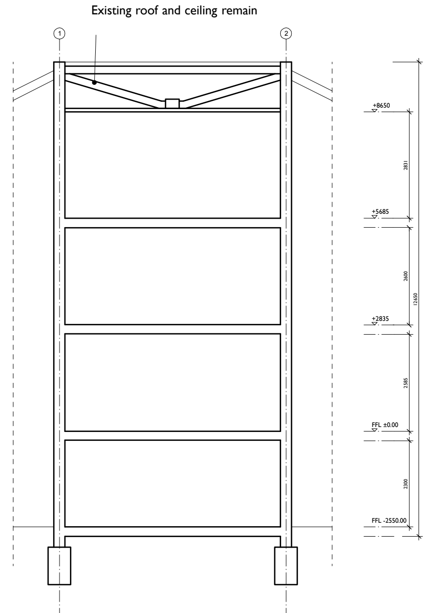
SECTION B
