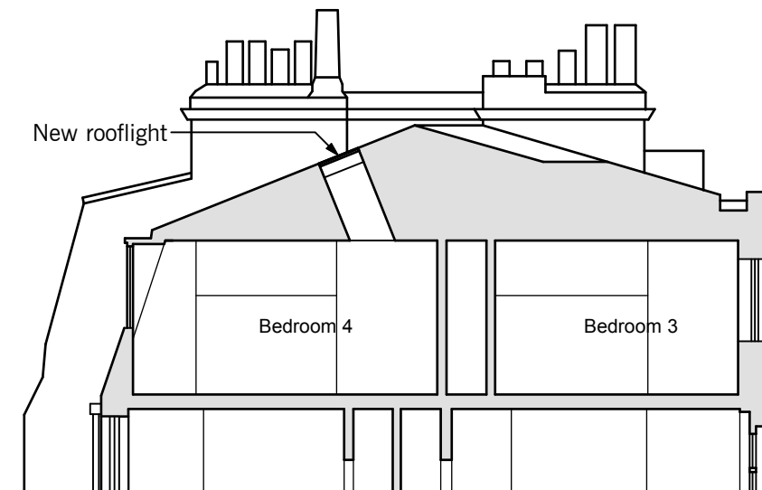
2. PROPOSED SECTION BB
