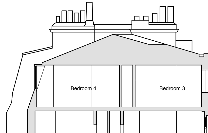
2. EXISTING SECTION BB
