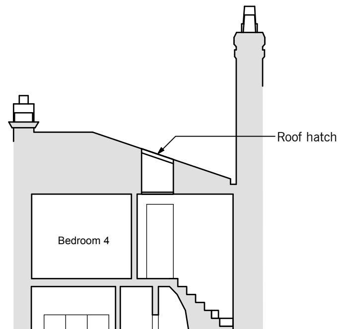
3. EXISTING SECTION CC
