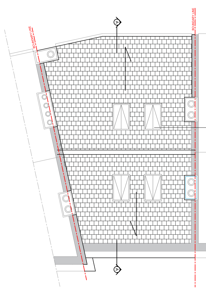
PROPOSED ROOF VIEW
