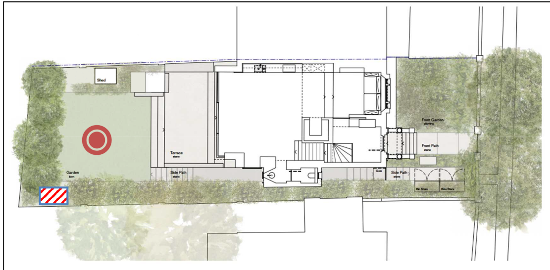
Figure 2.3 Site measurement position and proposed plant unit installation (Drawing Source: William Smalley)
