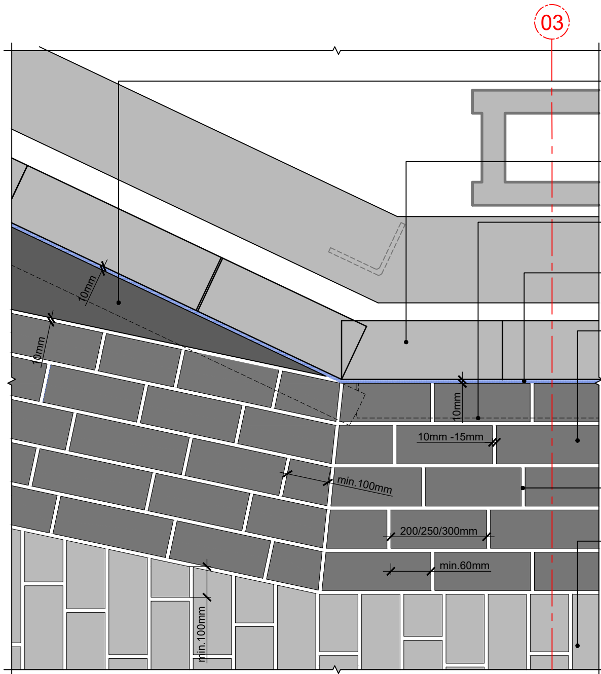
DETAIL PLAN OF GRANITE SETT STRETCHER COURSE TO CHILTON LANE SCALE: 1:10 @ A3
