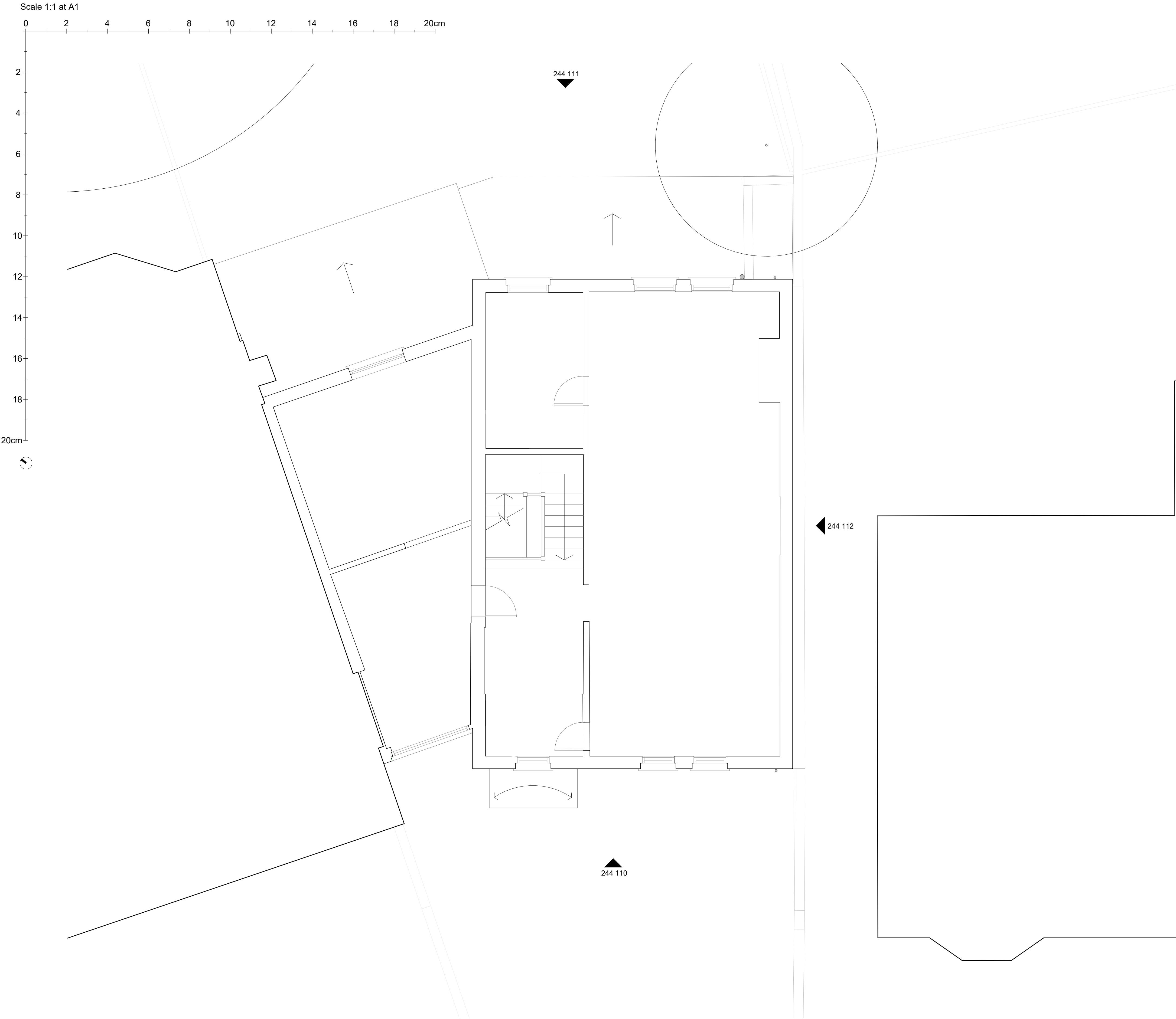
0102 EXISTING 2ND FLOOR PLAN
