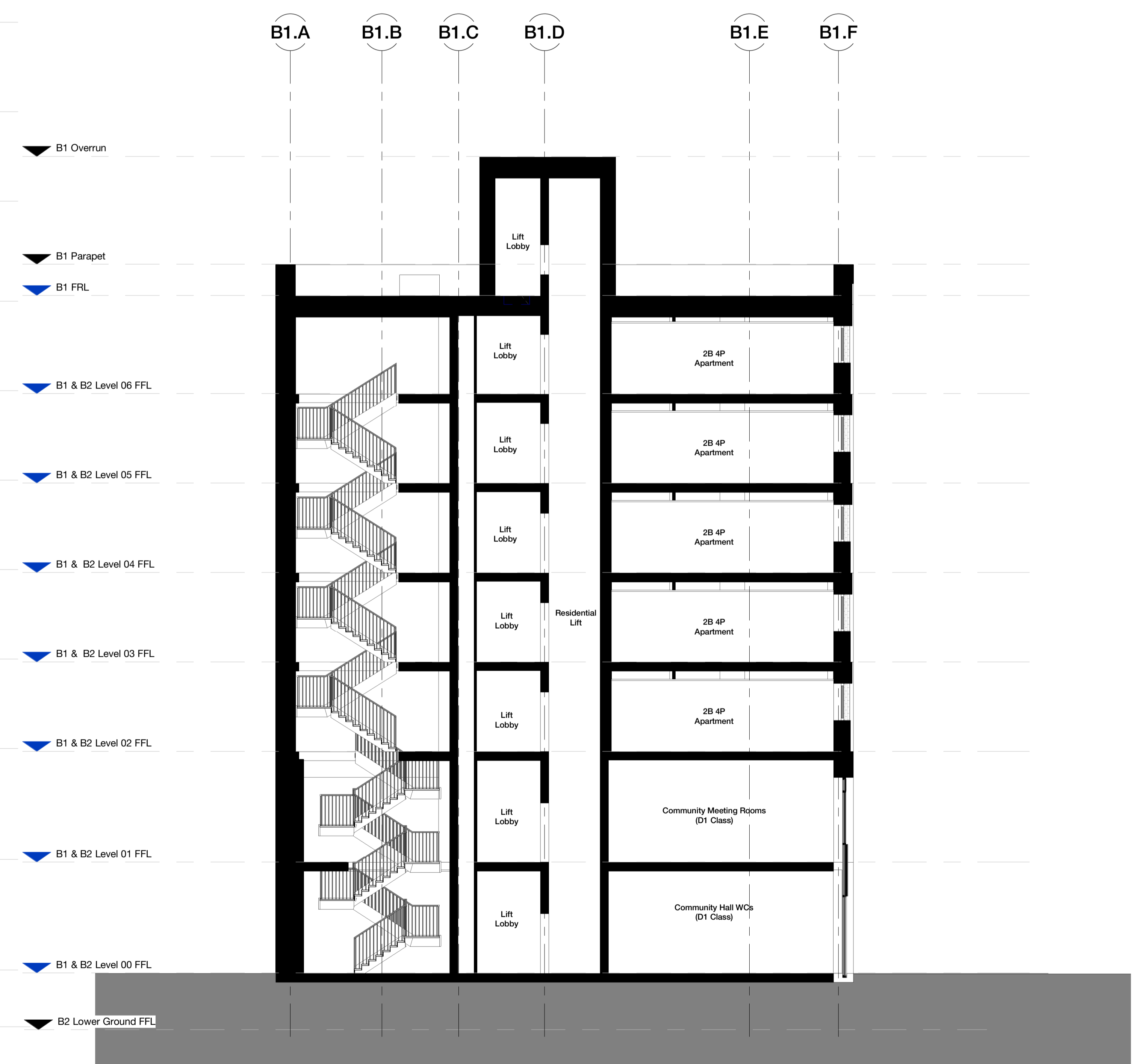
2 Short Section through B1 1 : 100
