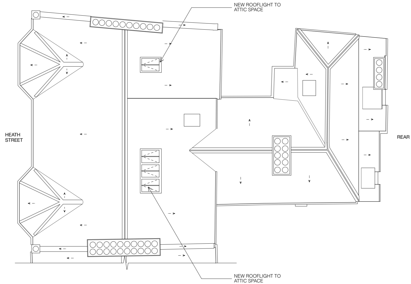
RP Proposed Roof Plan Scale: 1:100
