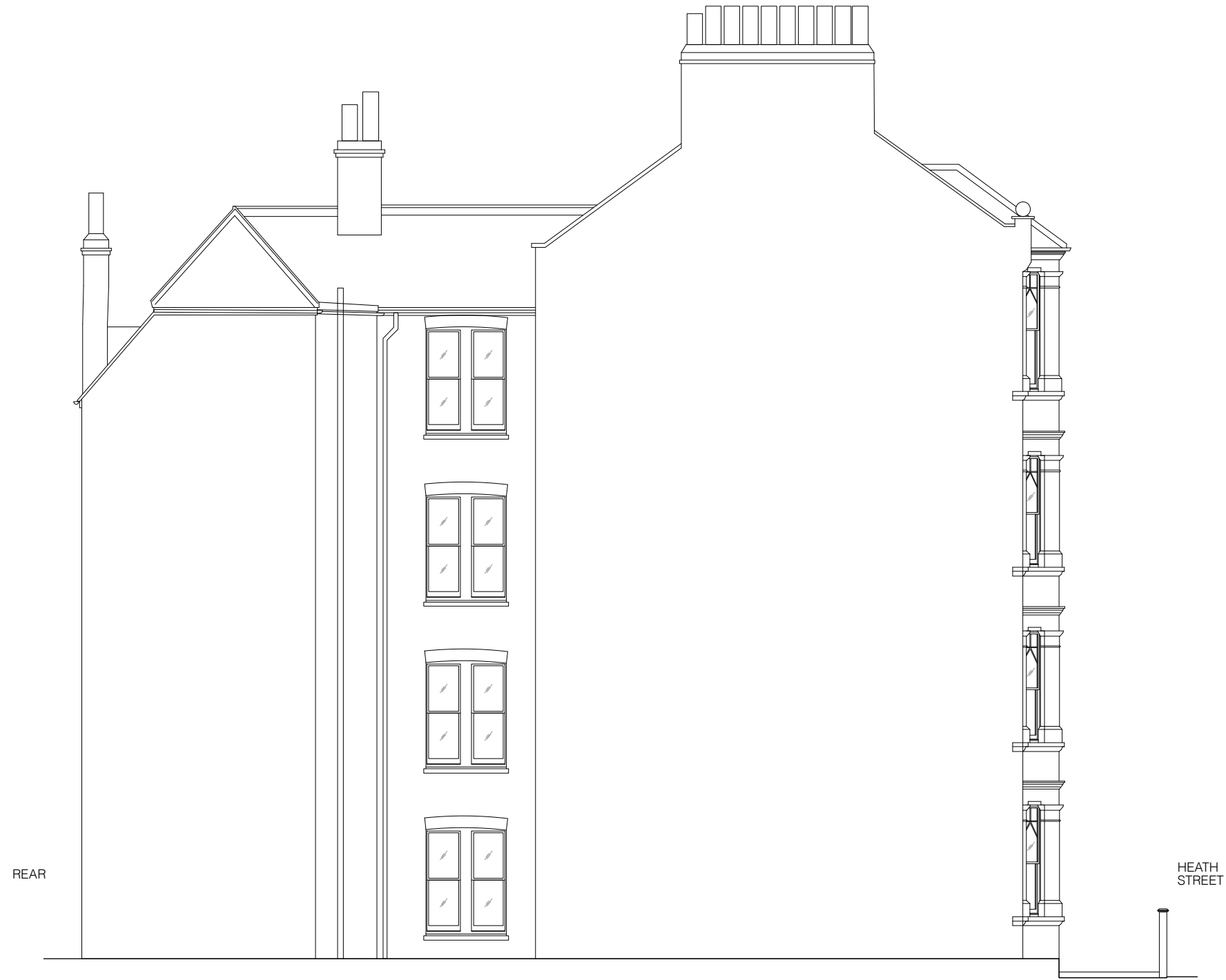
N External Elevation (North) Scale: 1:100
