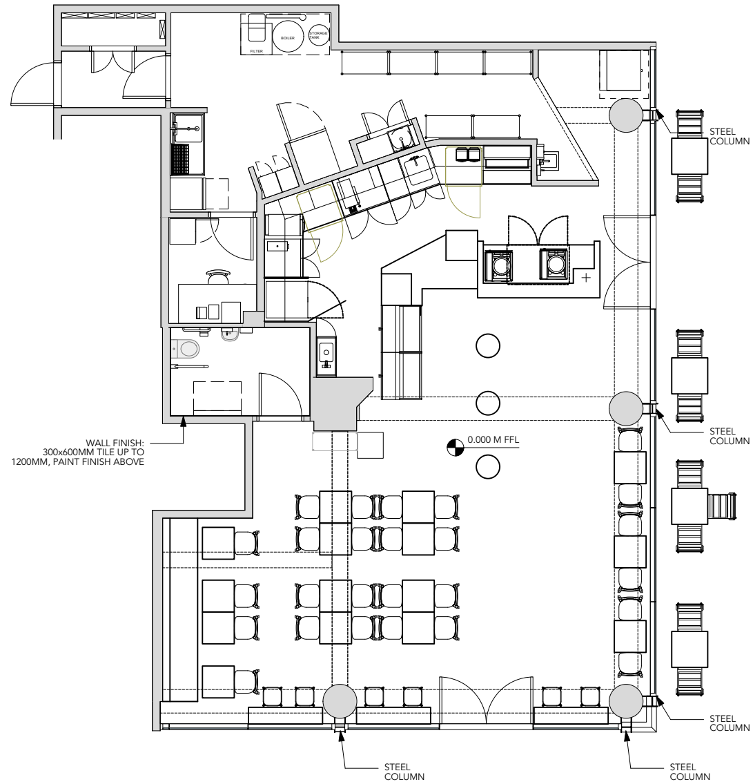
1 EXISTING FLOOR PLAN Scale: 1:100
