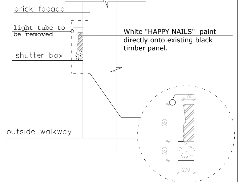
SECTION OF FRONT FACADE scale 1/100
