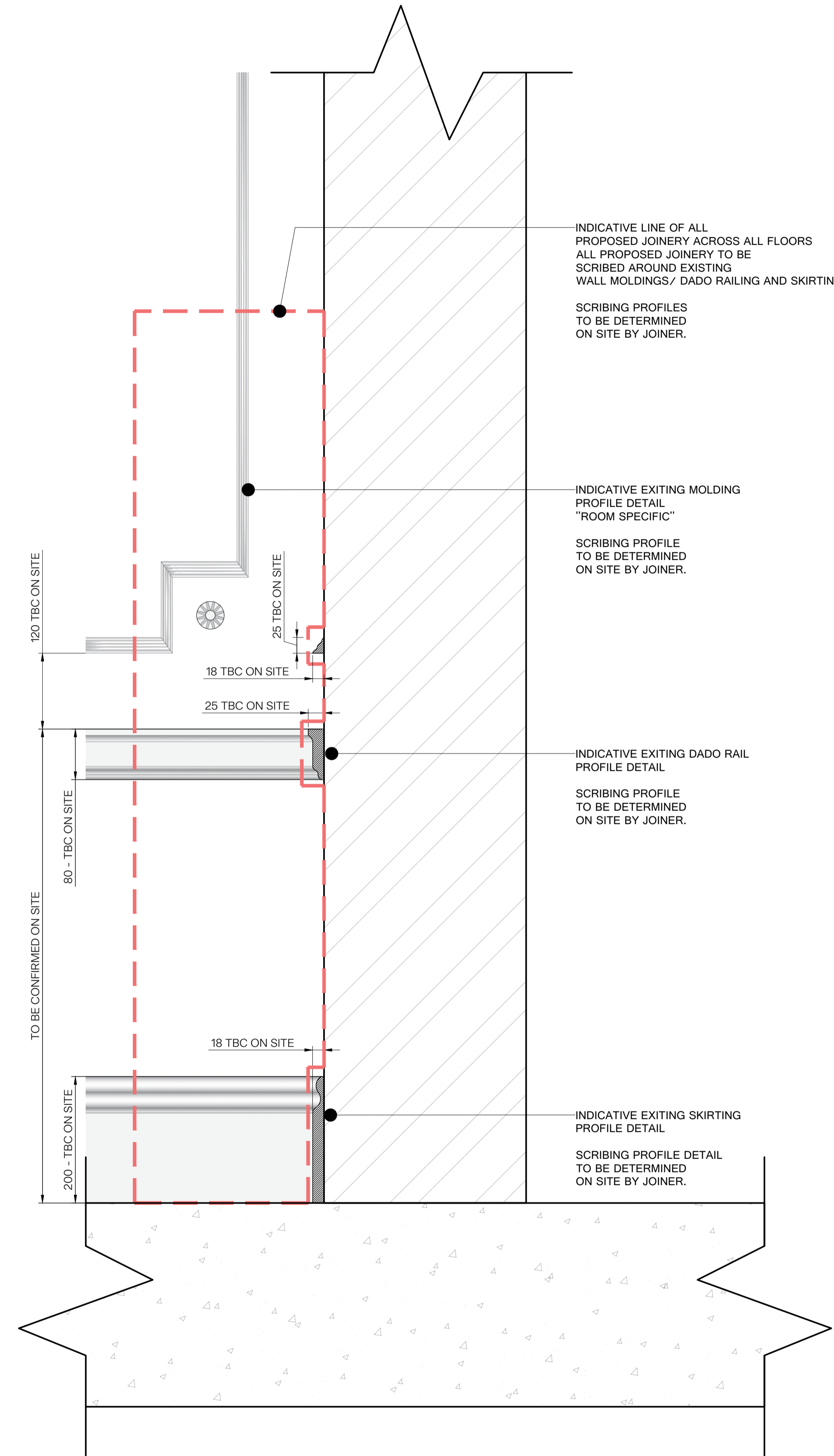
02 TYPICAL SKIRTING & DADO - SECTION A-A Scale: 1:5@A1
