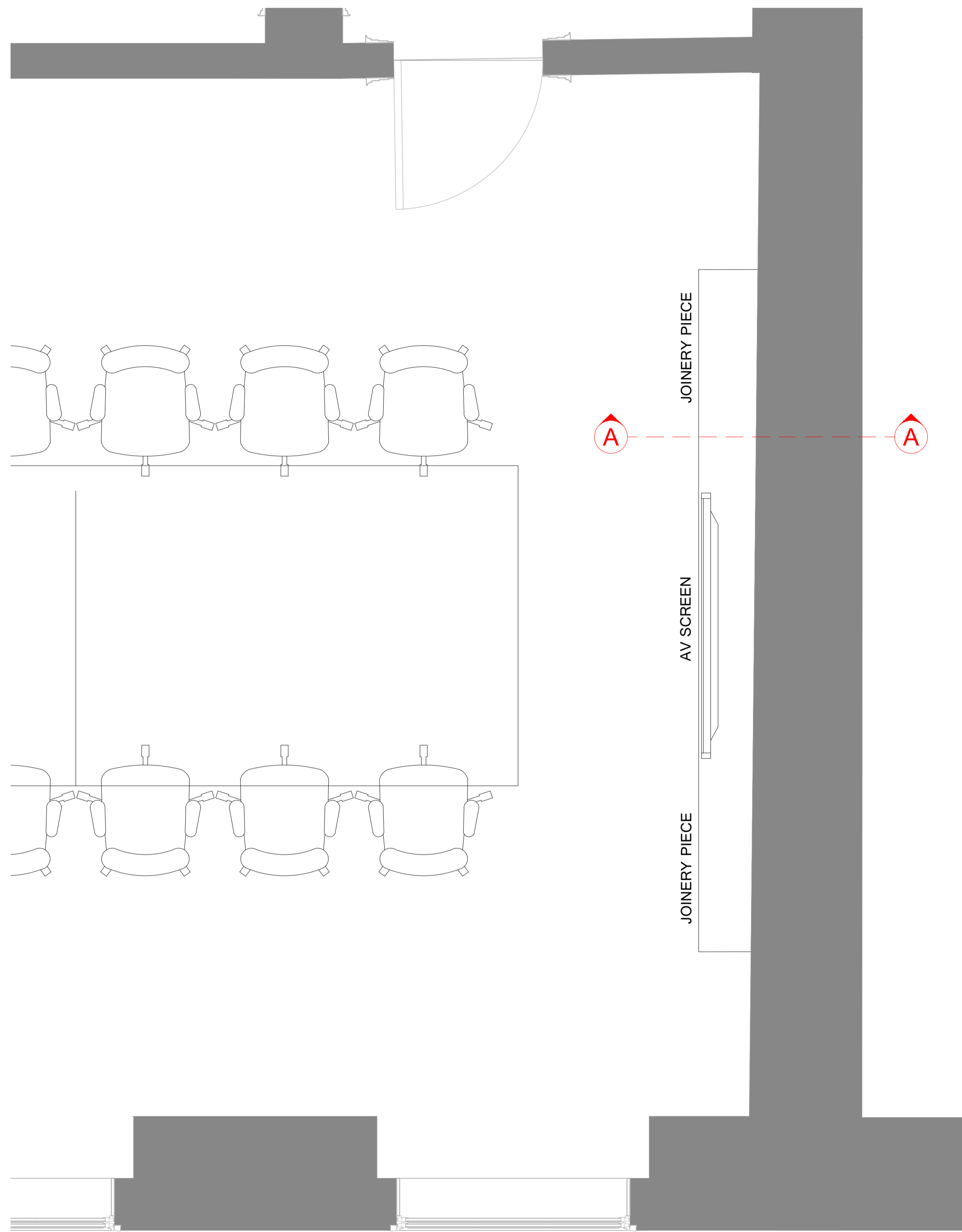
01 TYPICAL SKIRTING & DADO - PLAN VIEW Scale: 1:NTS@A1
