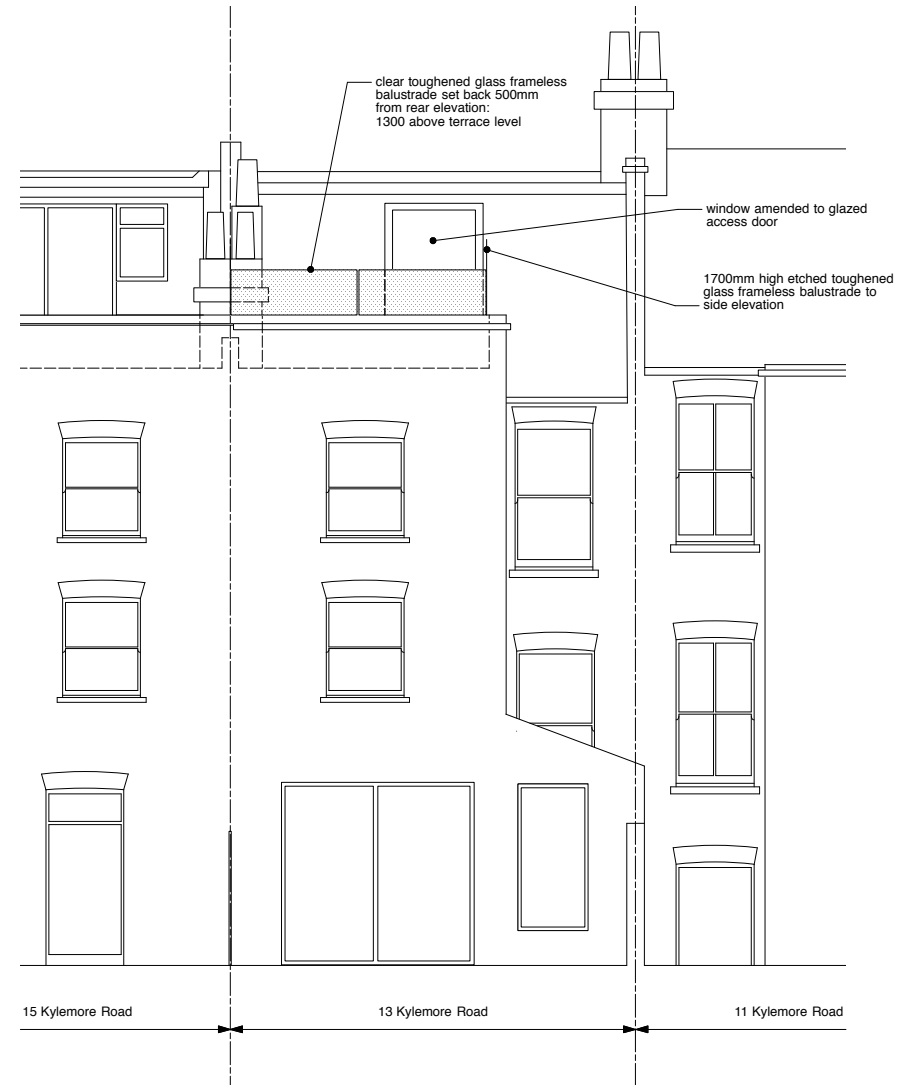
Rear Elevation B-B
