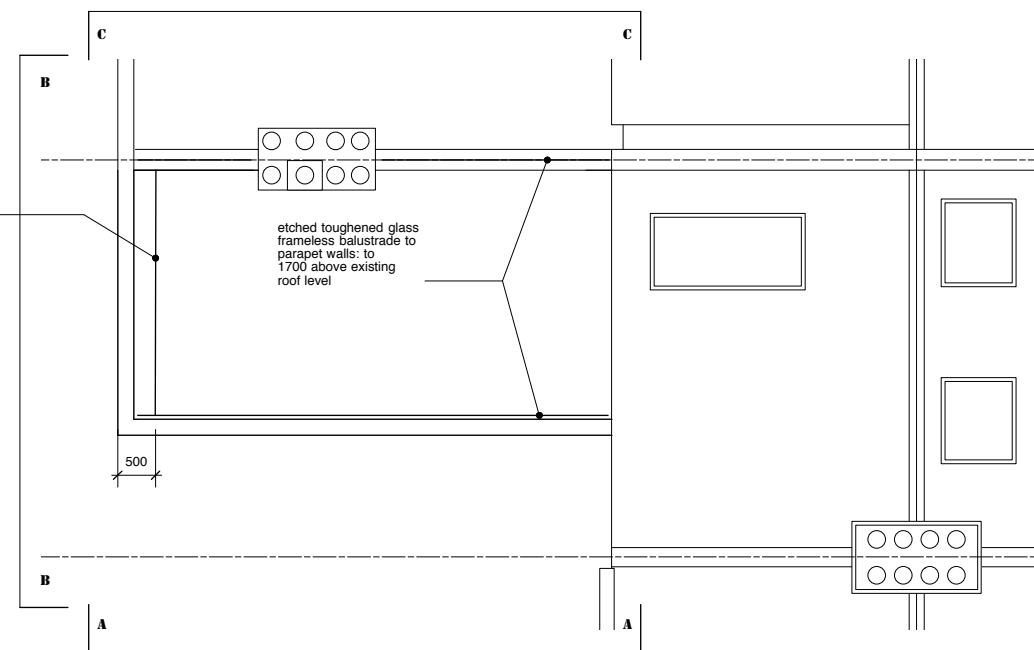
Roof Plan
