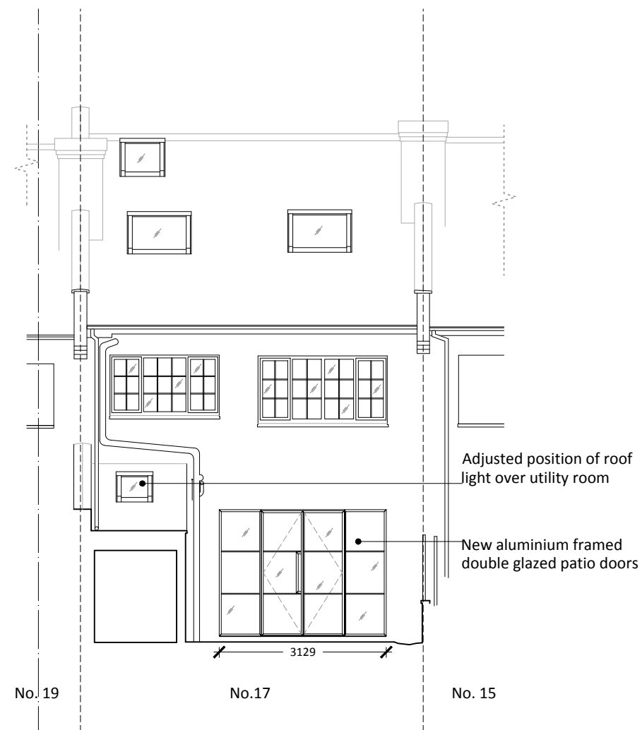
REAR ELEVATION
