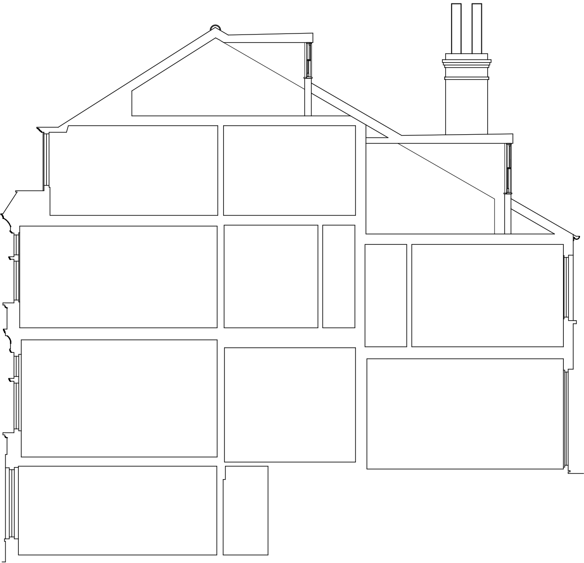
Section Through
