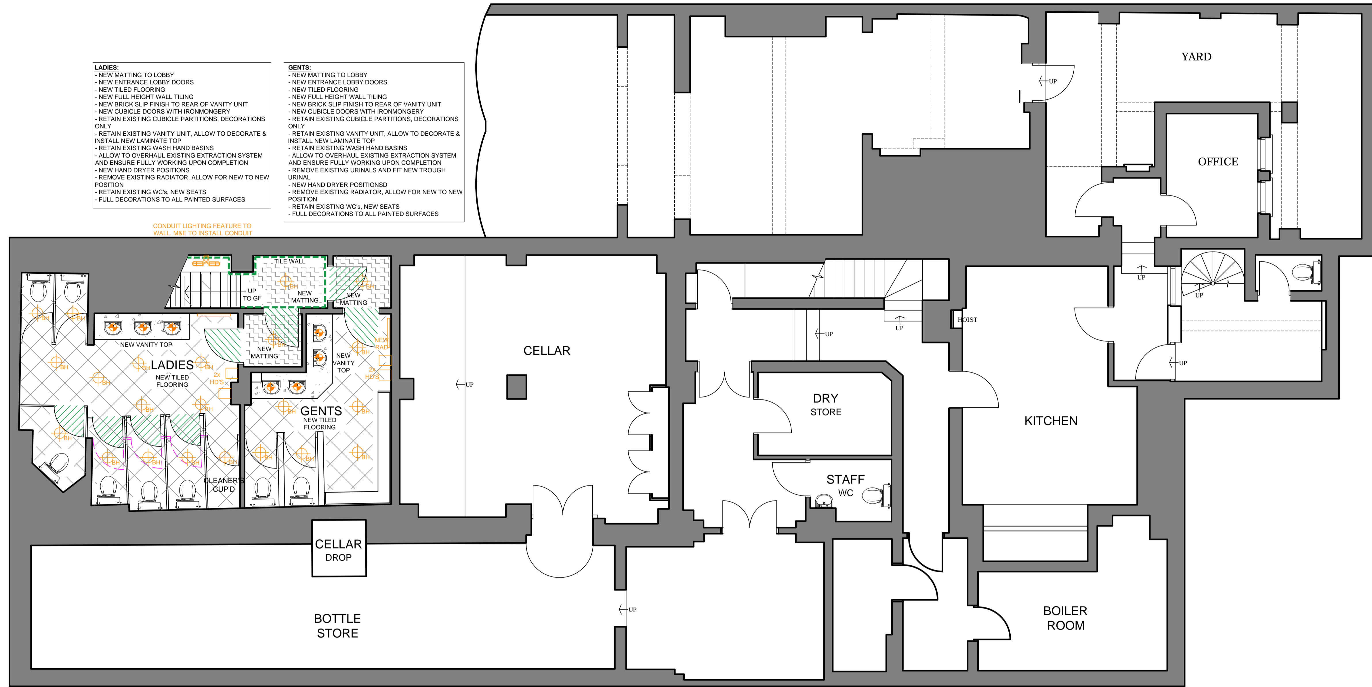
PROPOSED BASEMENT FLOOR 1:50 @ A1
