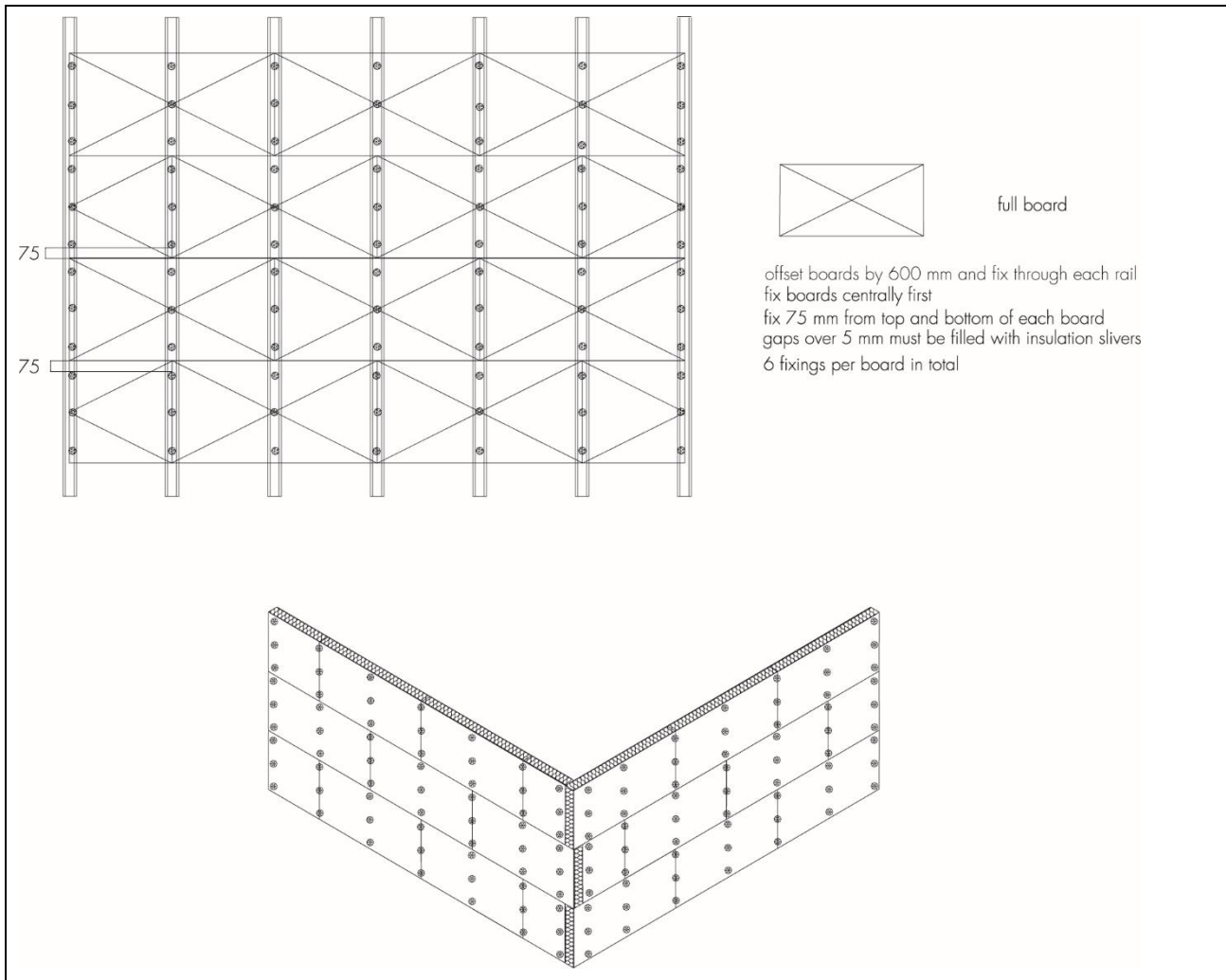
Figure 5 Arrangement of insulation slabs and typical fixing pattern
