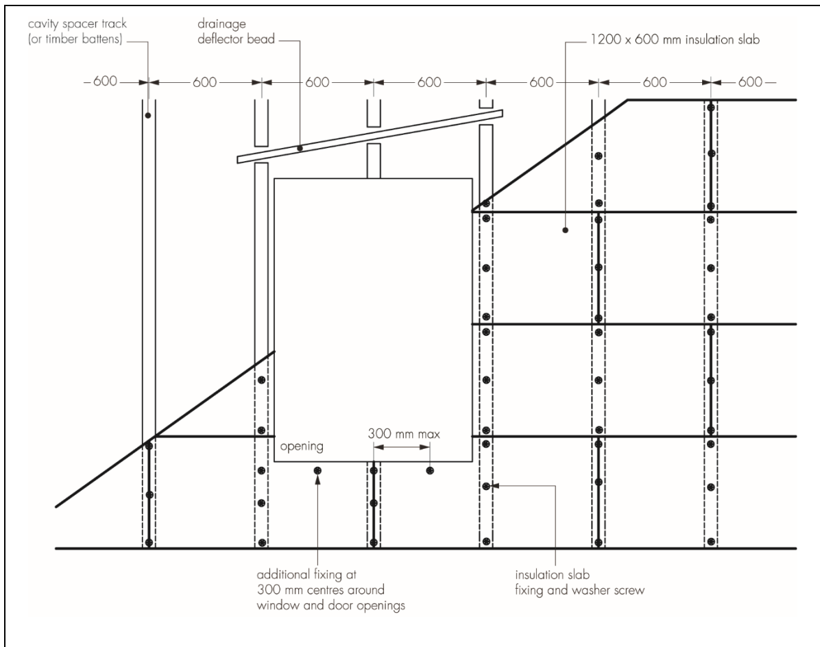
Figure 7 Typical opening details showing deflection channel
