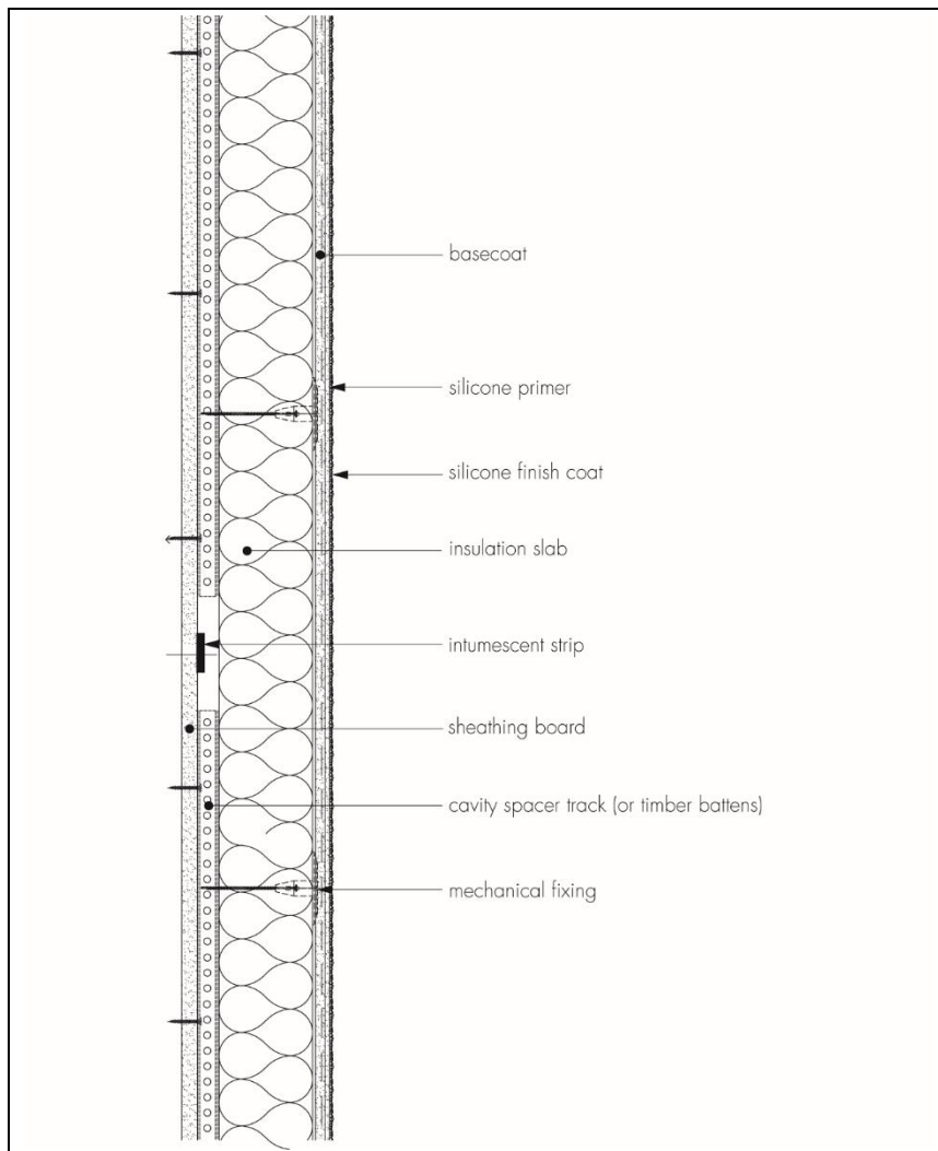
Figure 3 Fire barriers
