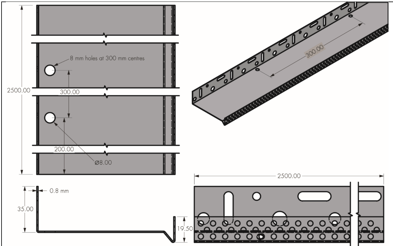
Figure 4 Typical section of base rail
