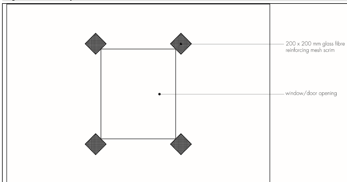
Figure 9 Corner reinforcement
