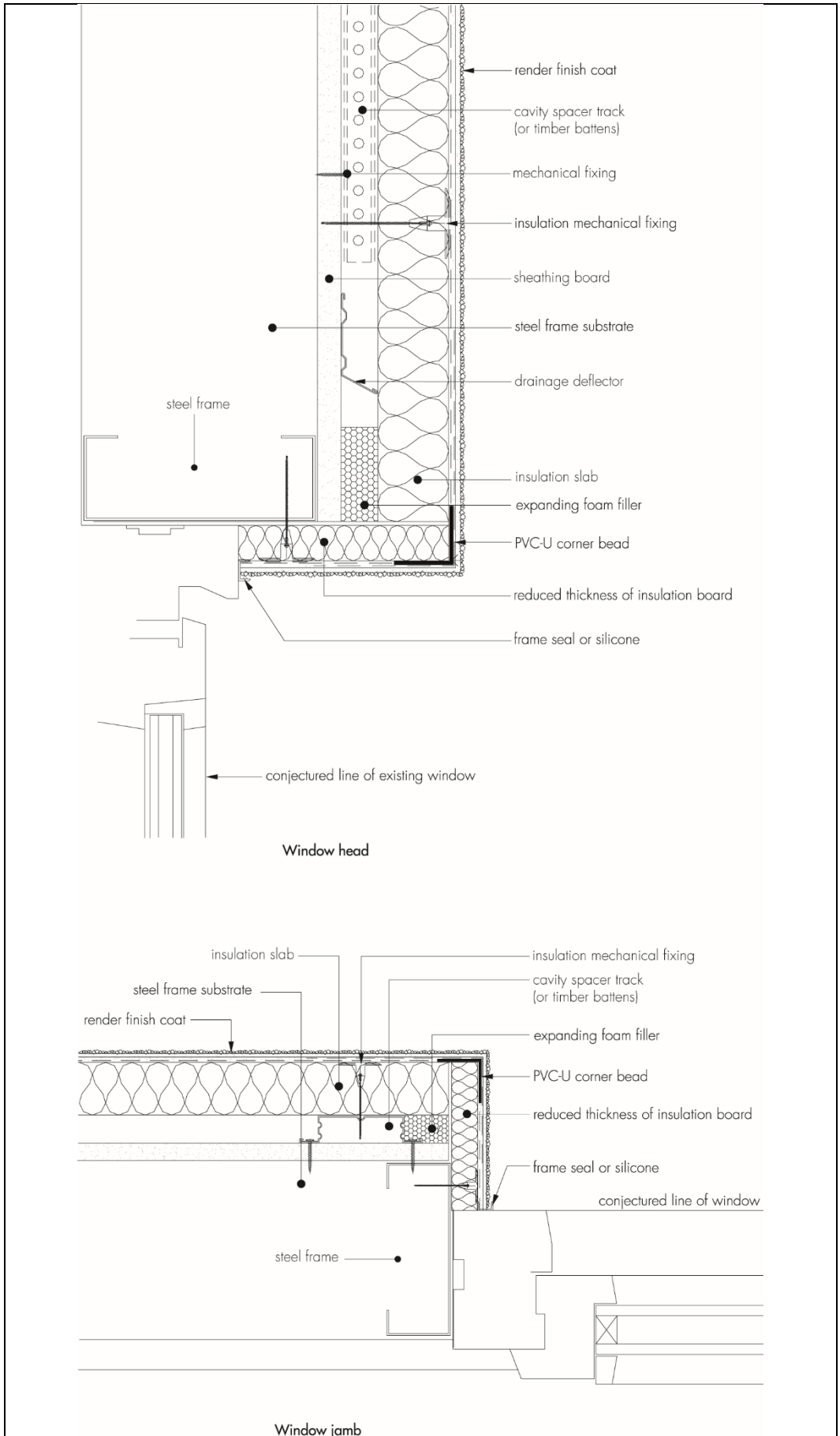
Figure 11 Typical window head and jamb details
