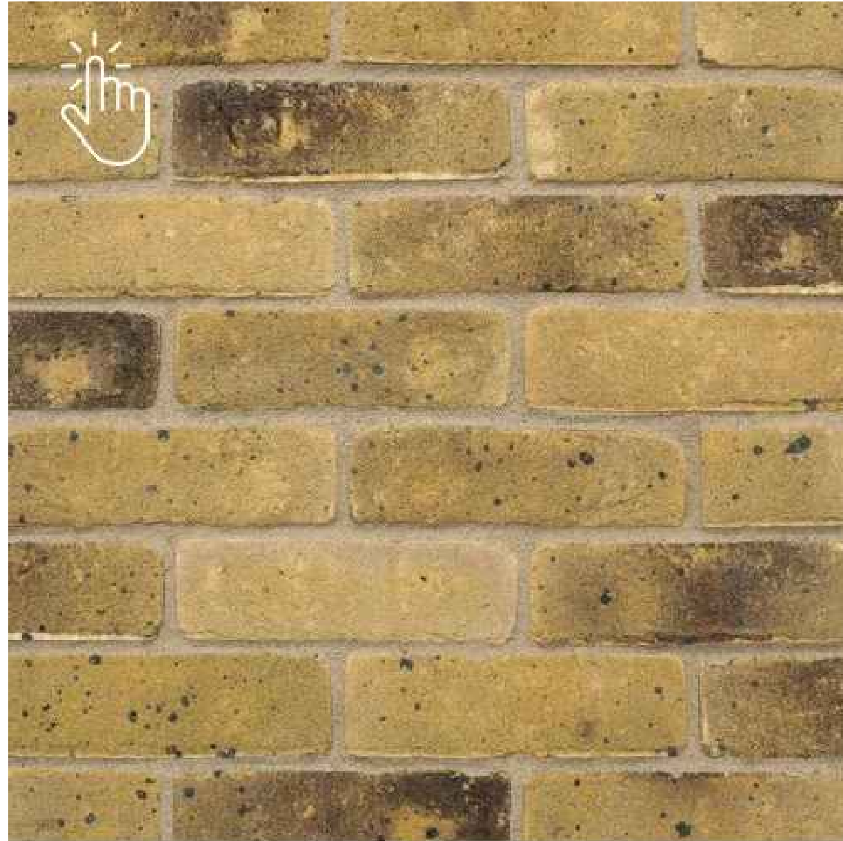
Spec: Facing brickwork for rear elevation extension and new 2 storey dwelling Supplier: Wienerberger or equal Type: Smeed Dean Weathered yellow Stock Coursing, pointing & bonding: to match existing
