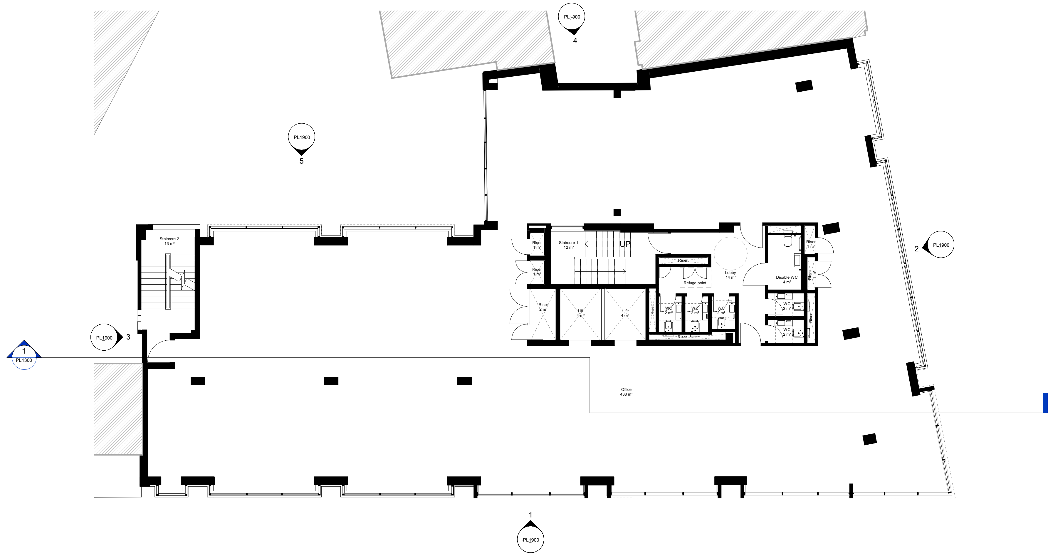
1 02 - Second Floor 1 : 100
