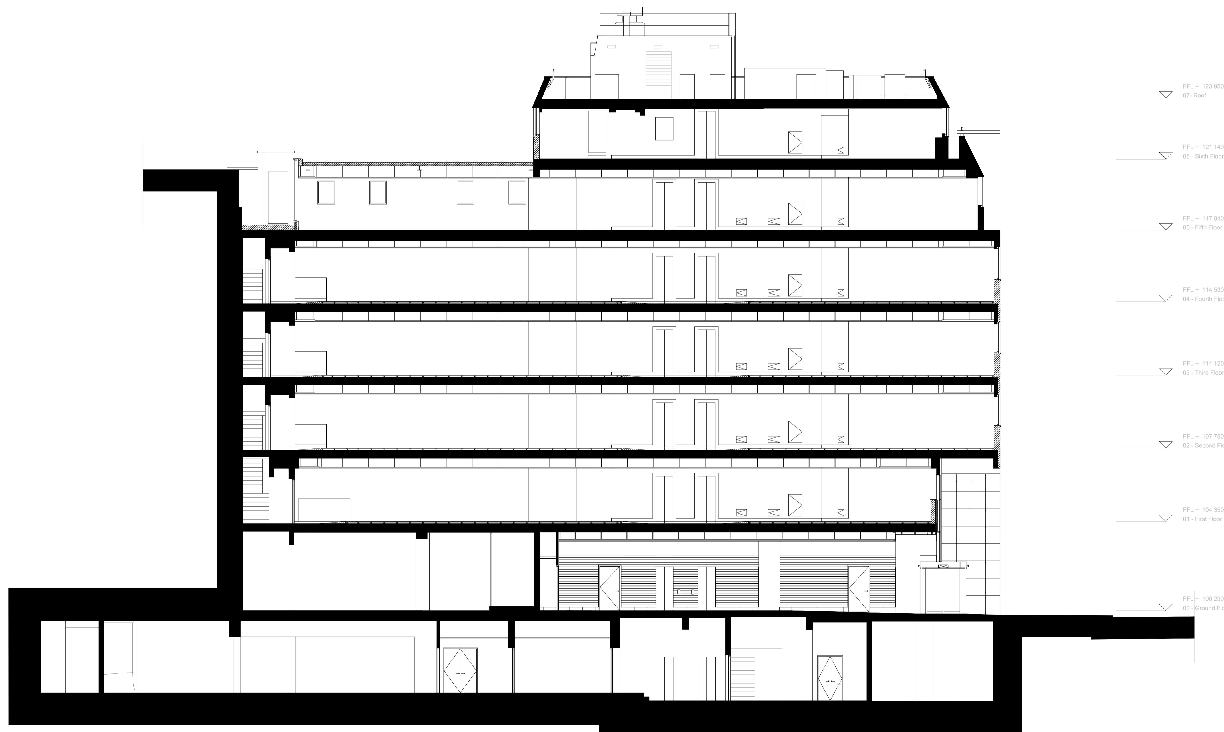
1 Section A-A - Existing working 1 : 100
