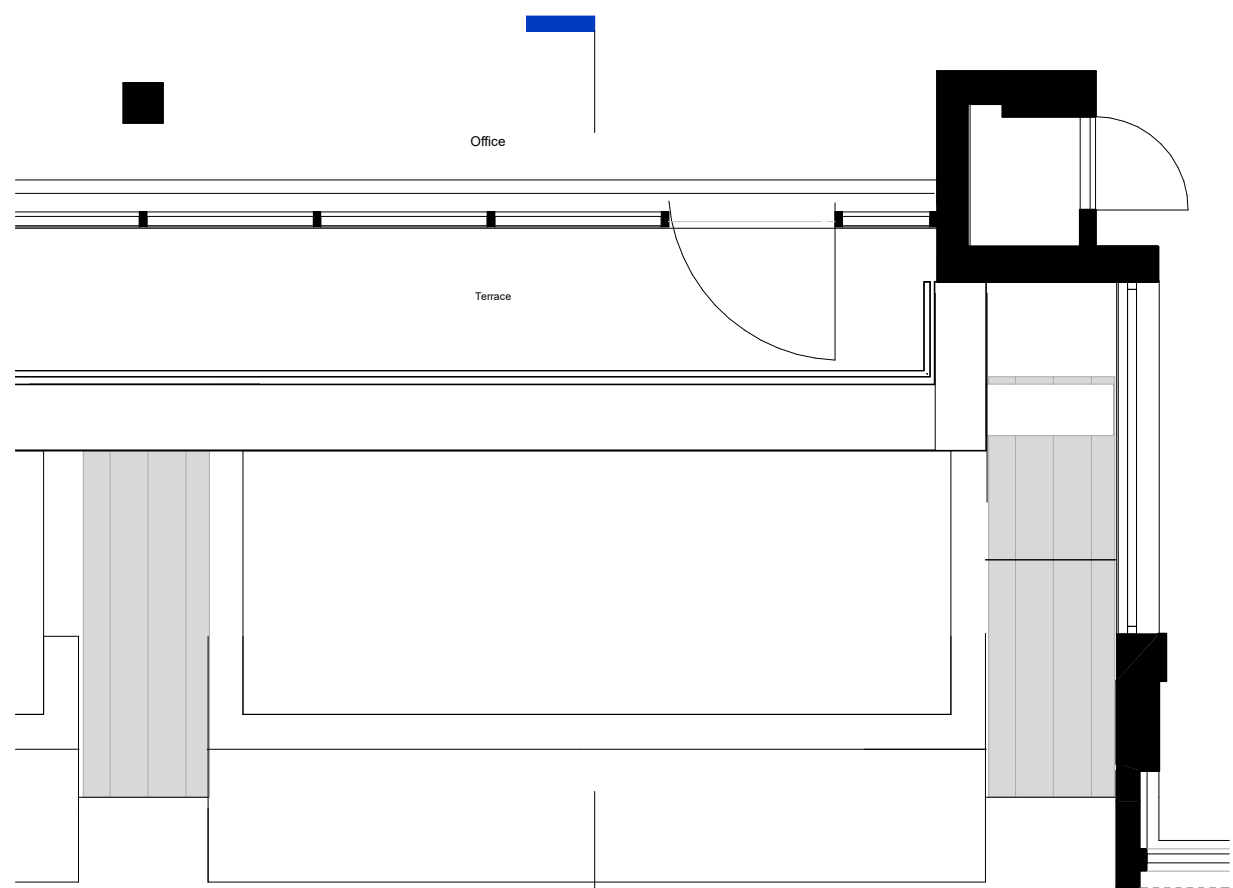
6 Fifth Floor Level - Gate/Terrace Detail 1 : 50
