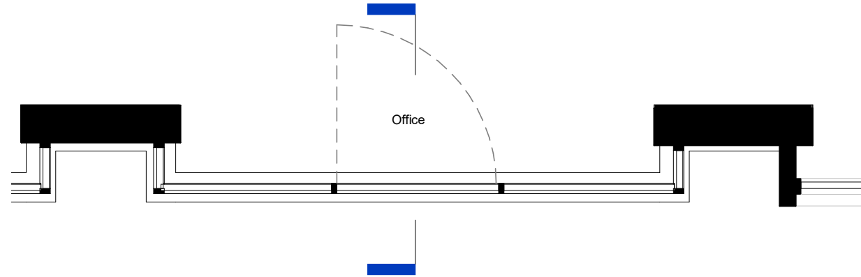
4 Second Floor Level - Gate/Terrace Detail 1 : 50
