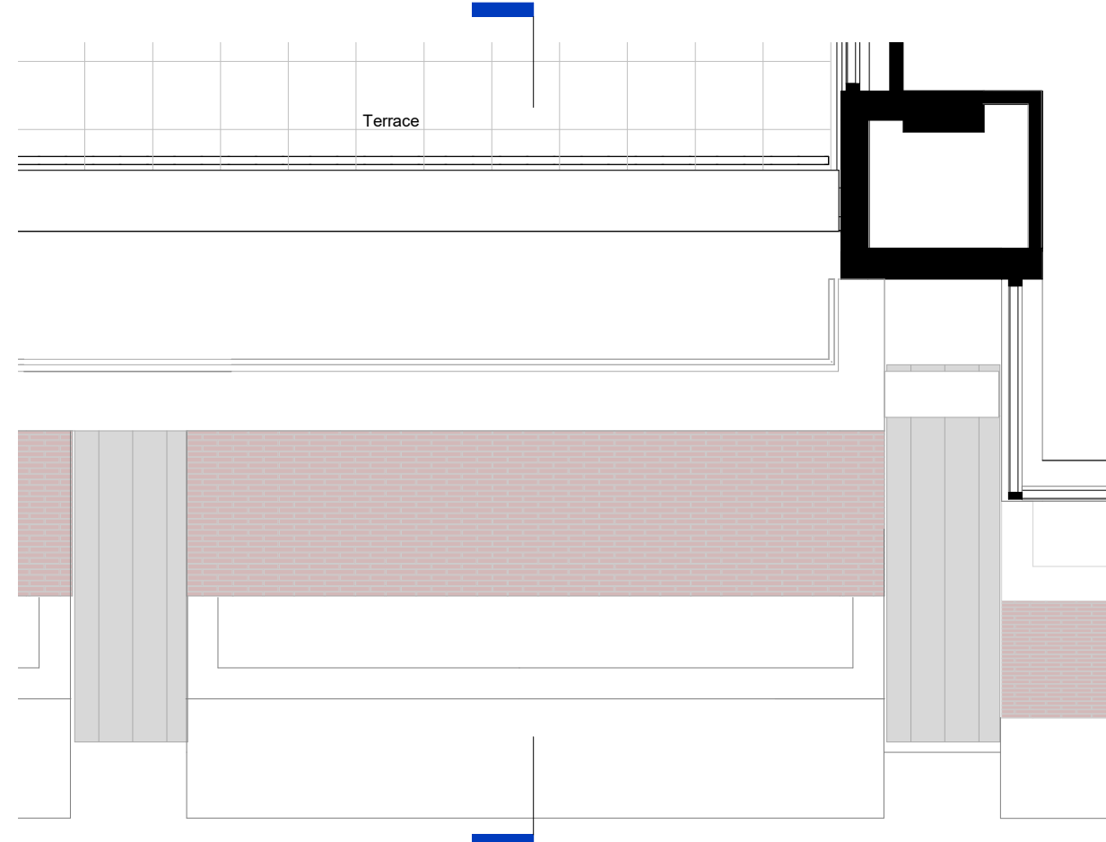
5 Sixth Floor Level - Gate/Terrace Detail 1 : 50
