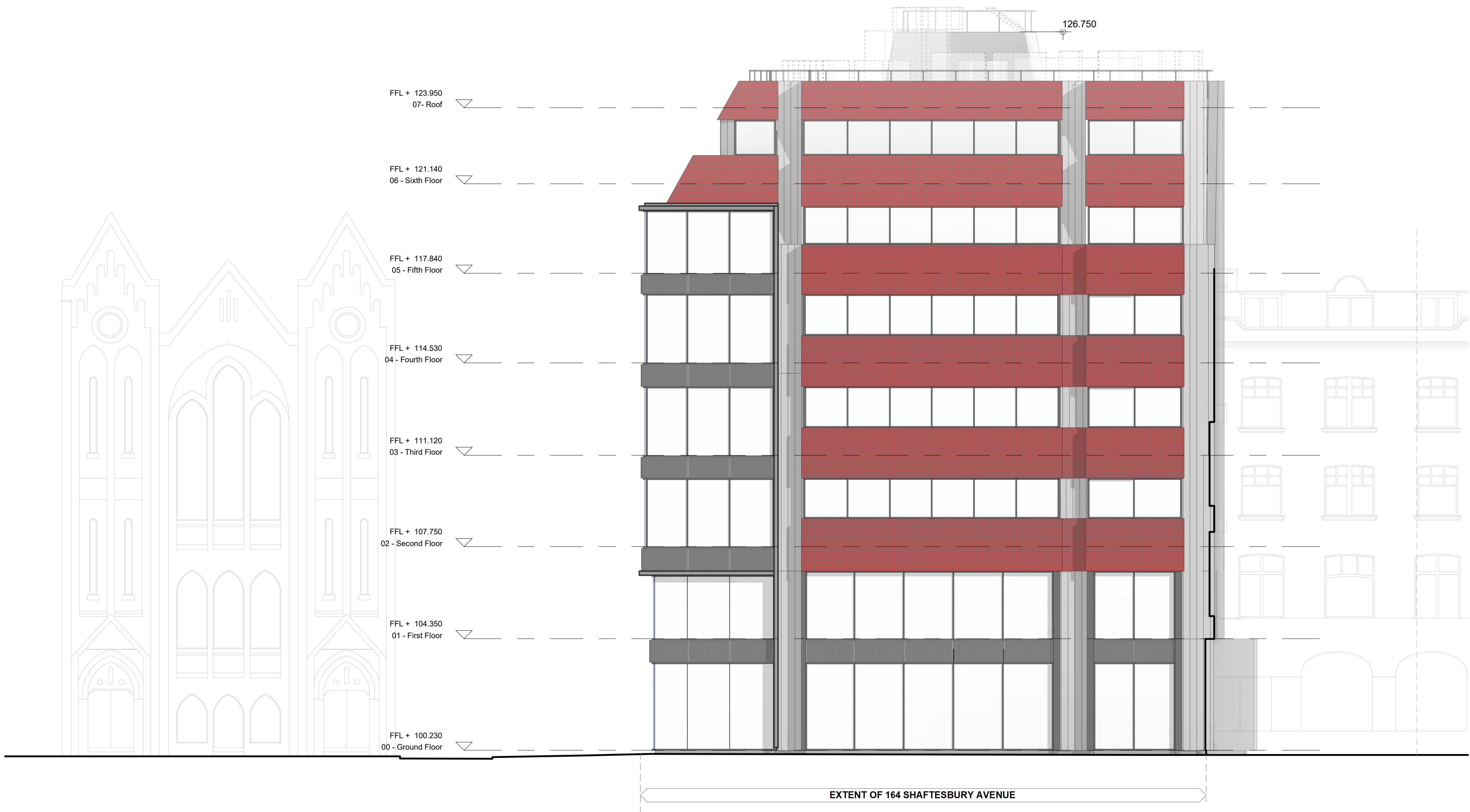
1 Proposed North-West Elevation 1 : 100
