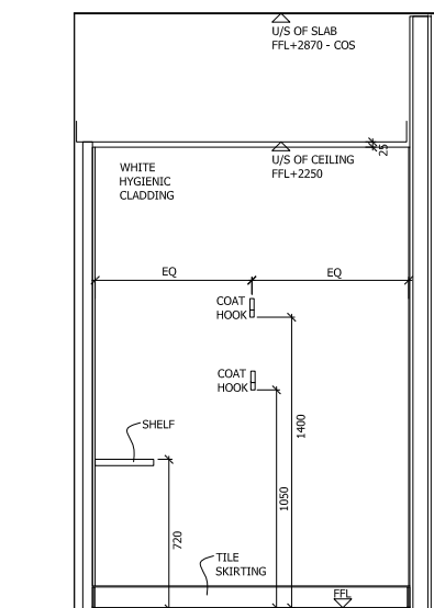
B ACCESSIBLE WC ELEVATION B 1:20
