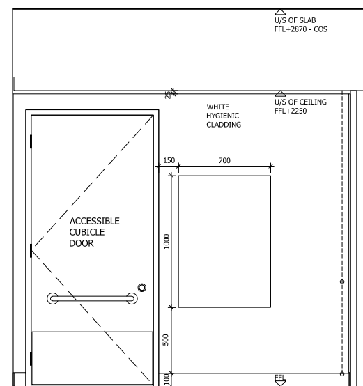
C ACCESSIBLE WC ELEVATION C 1:20
