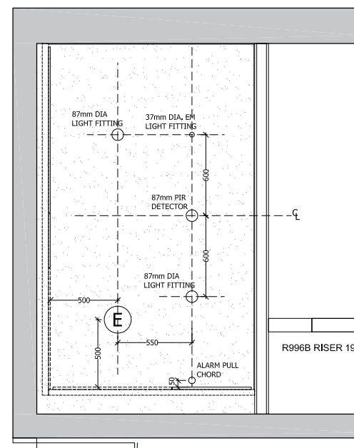
2 ACCESSIBLE WC CEILING PLAN 1:20
