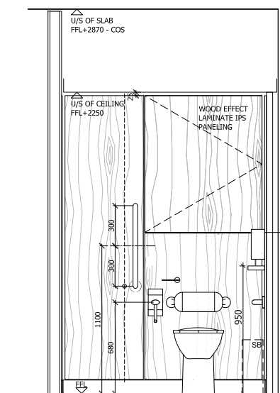
D ACCESSIBLE WC ELEVATION D 1:20
