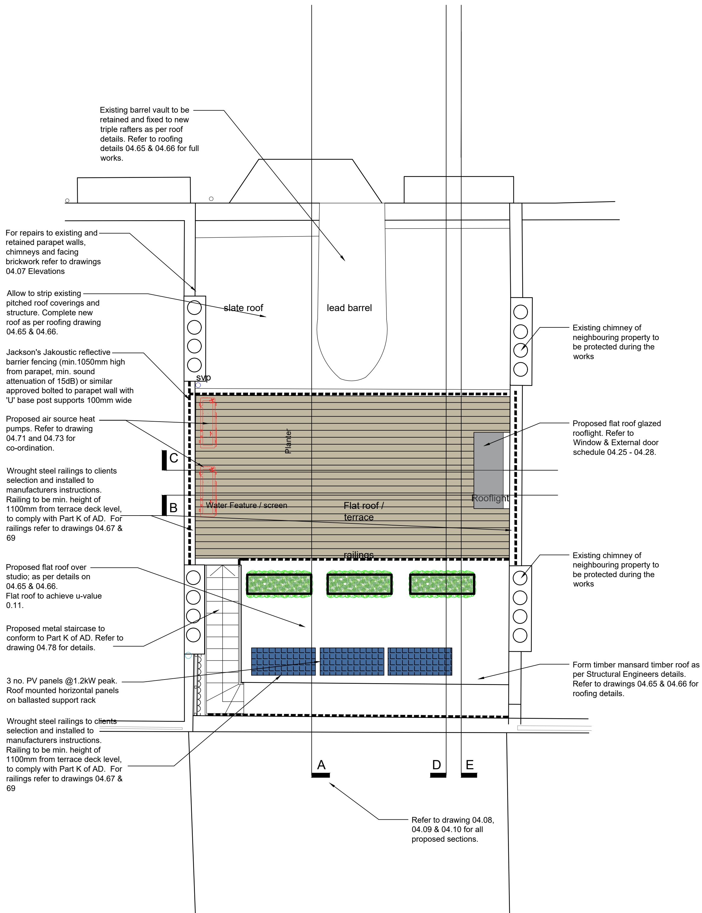
Roof Level - General Arrangement Scale 1:50
