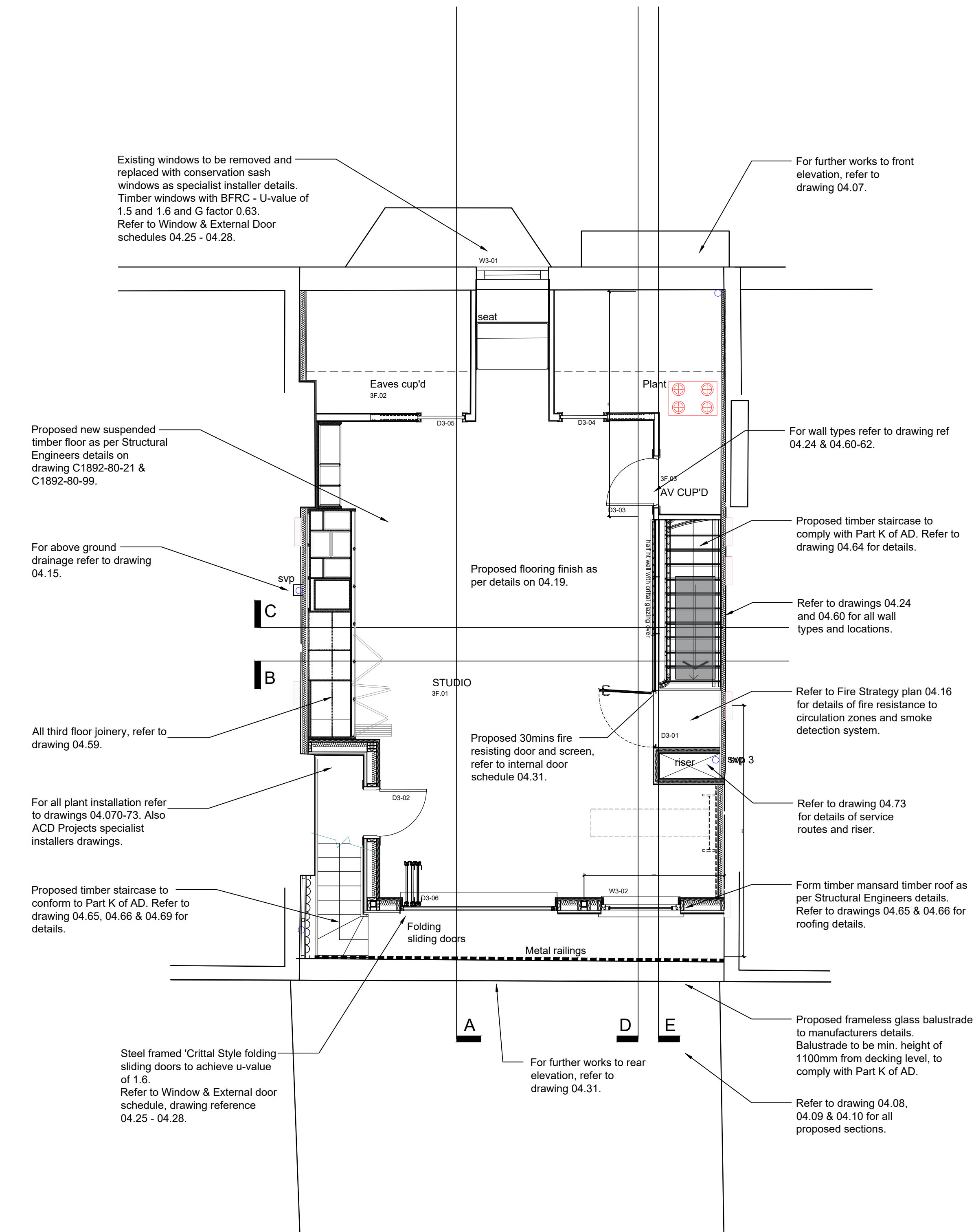
Third Floor - General Arrangement Scale 1:50
