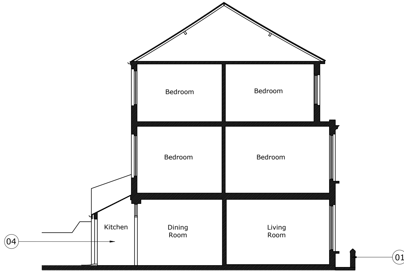
01 Existing_Section A 01 200 Scale 1:100@A3
