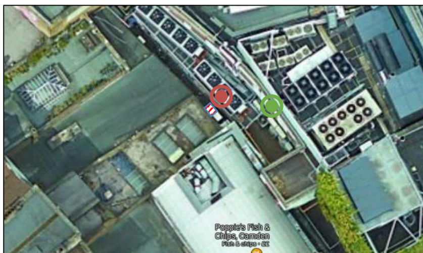
Figure 2.2 Site measurement position, identified receiver and proposed plant unit installation (Image Source: Google Maps)
