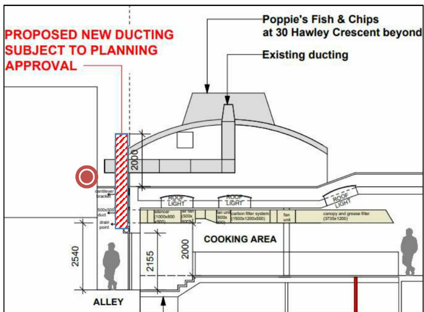
Figure 2.3 Site measurement position and proposed plant unit installation (Image Source: Ganguly Architects Ltd.)
