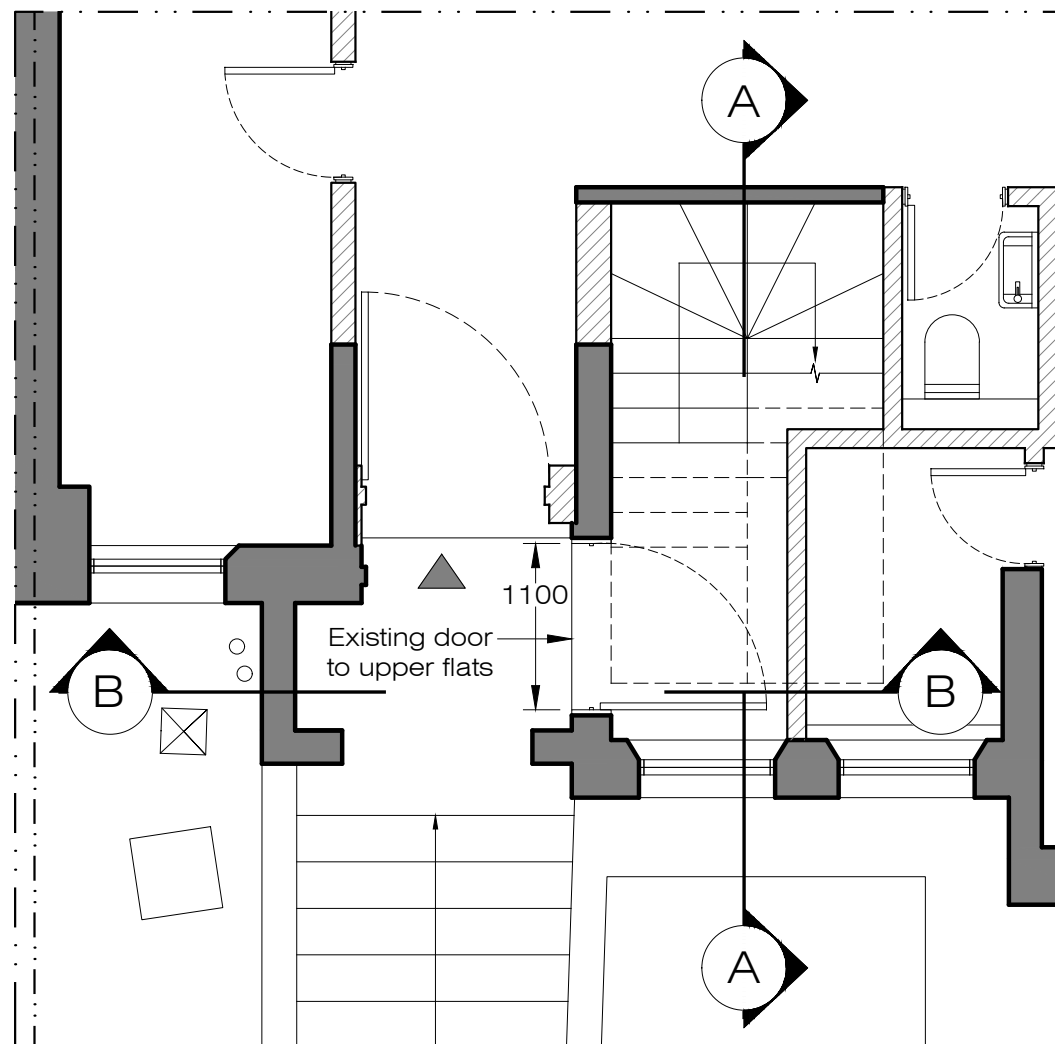
X EXISTING Upper Ground Floor Plan 1:50@A3
