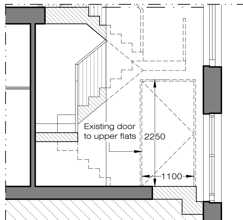
X EXISTING Section AA 1:50@A3
