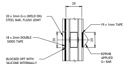
G+s Detail Outside Flush Joint with Trapezoidal Applied Bar
