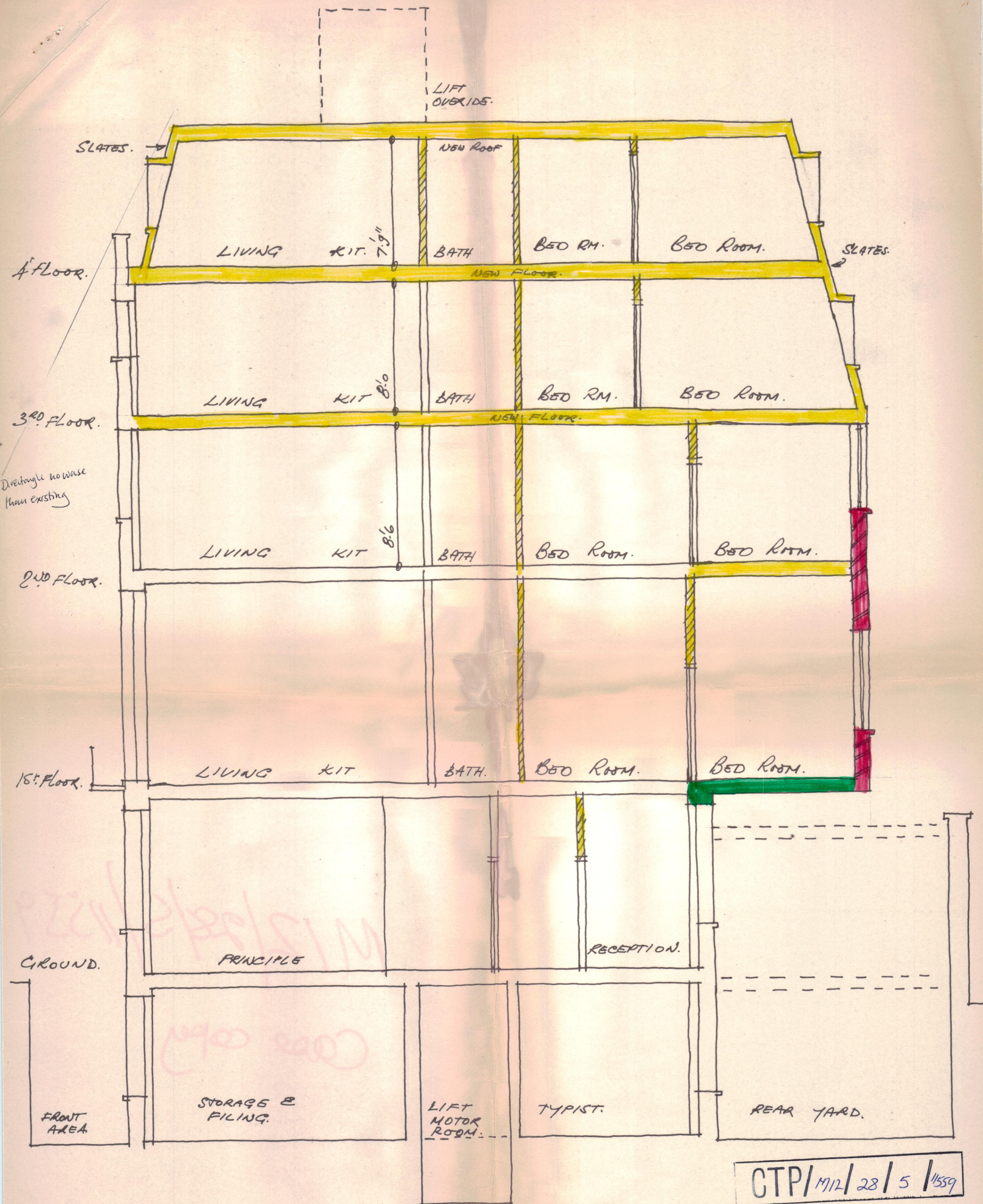
CROSS SECTION.
