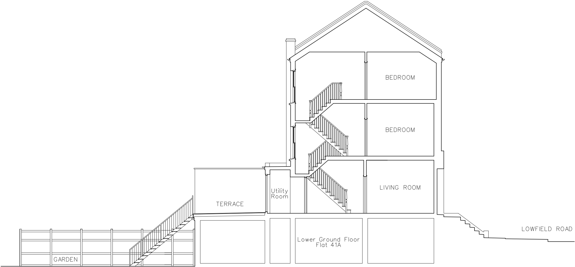
1. BUILDING CROSS SECTION (Section A)
